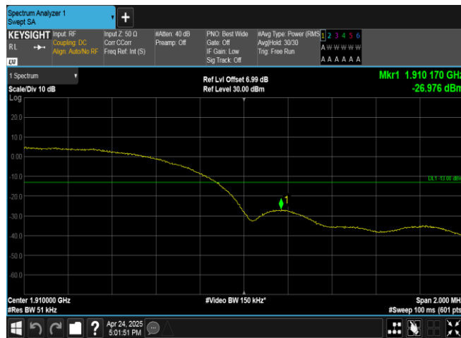
Band2-9538-4-PASS
