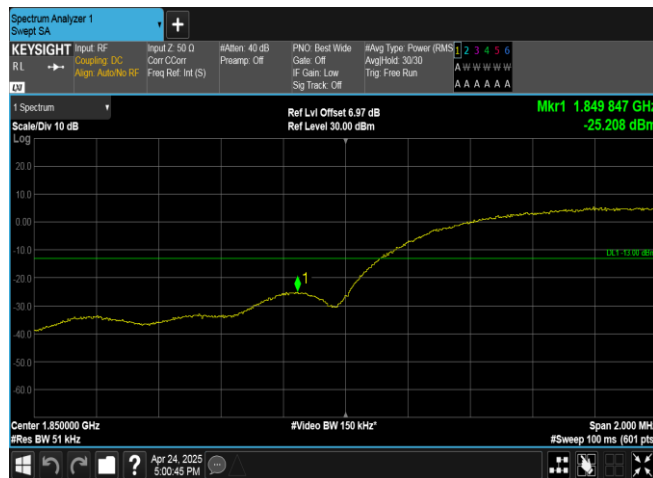
Band2-9262-3-PASS
