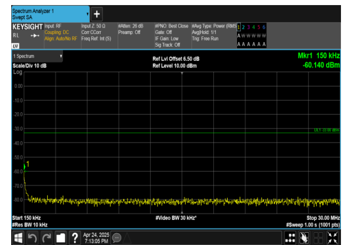
Band4-1513-0.15~30MHz-PASS
