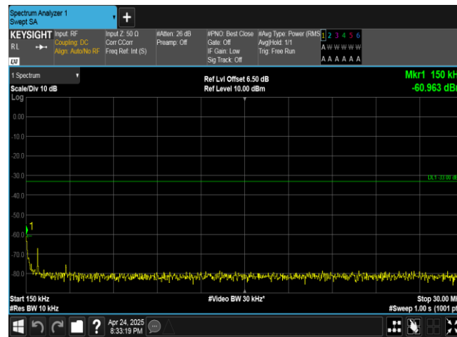
Band4-1312-3-0.15~30MHz-PASS
