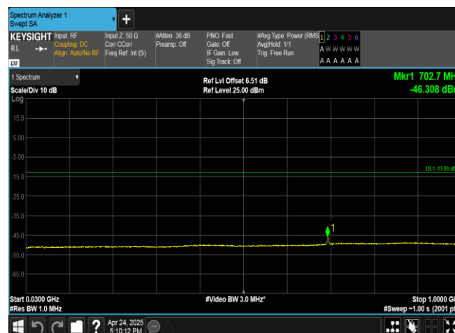
Band2-9538-4-30~1000MHz-PASS
