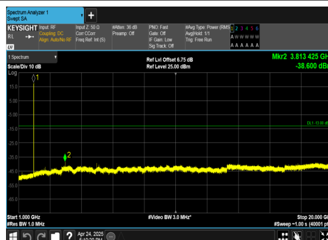
Band2-9538-4-1000~20000MHz-PASS
