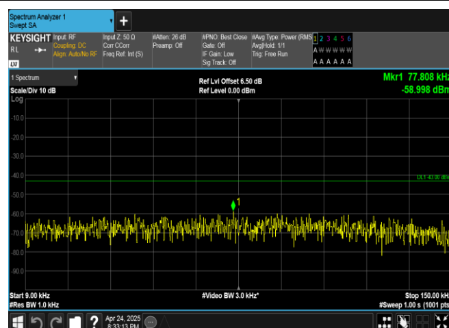
Band4-1312-3-0.009~0.15MHz-PASS
