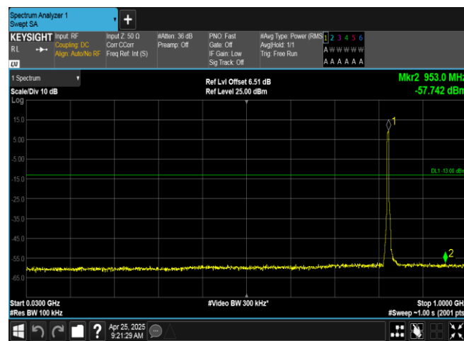
Band5-4182-2-30~1000MHz-PASS
