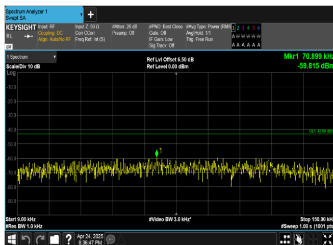
Band4-1513-4-0.009~0.15MHz-PASS
