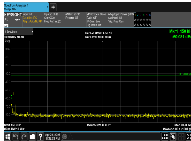
Band4-1513-4-0.15~30MHz-PASS
