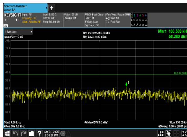
Band4-1513-3-0.009~0.15MHz-PASS
