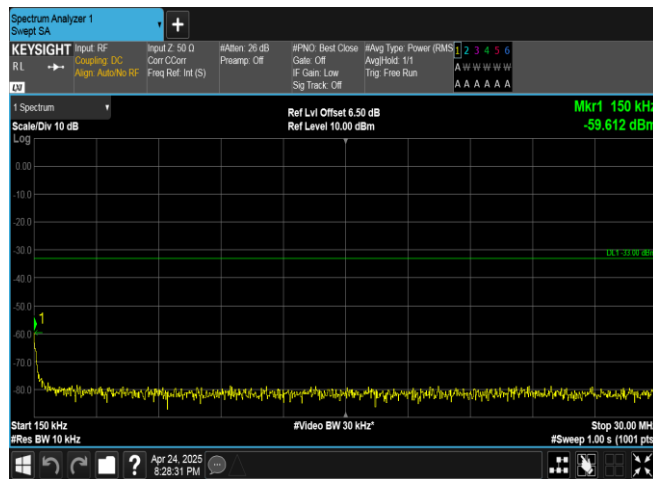
Band4-1312-1-0.15~30MHz-PASS
