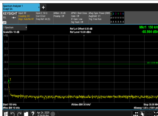
Band4-1413-1-0.15~30MHz-PASS
