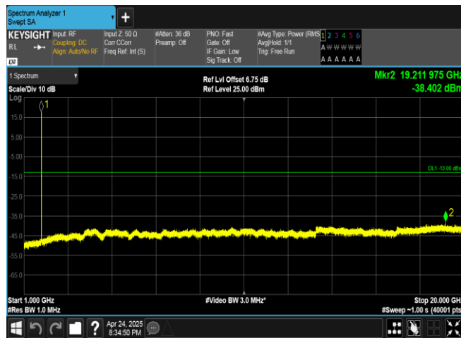
Band4-1513-3-1000~20000MHz-PASS
