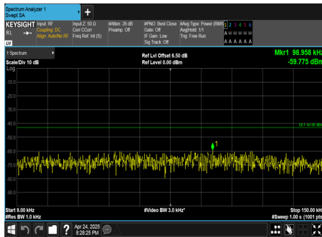
Band4-1312-1-0.009~0.15MHz-PASS
