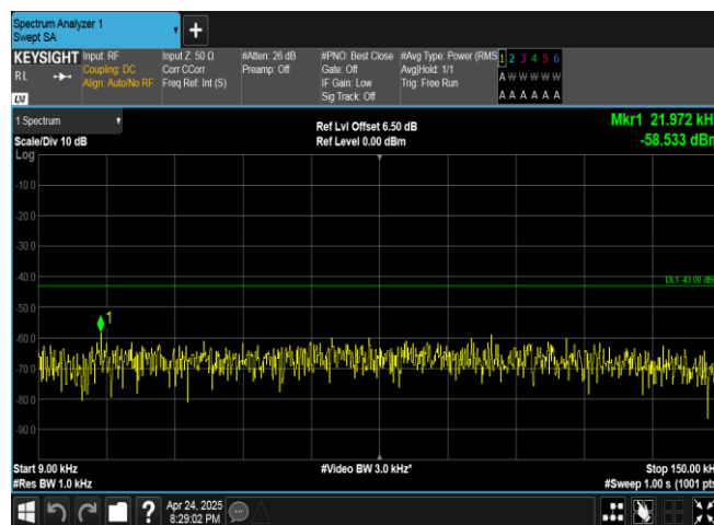
Band4-1413-1-0.009~0.15MHz-PASS
