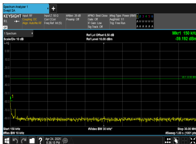
Band4-1413-4-0.15~30MHz-PASS
