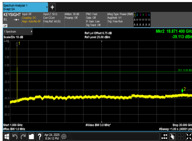
Band4-1413-3-1000~20000MHz-PASS
