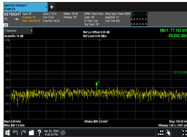
Band4-1312-4-0.009~0.15MHz-PASS
