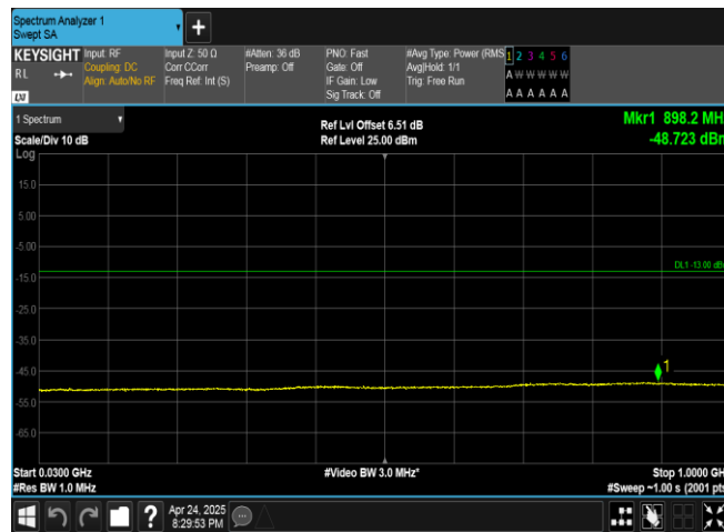
Band4-1513-1-30~1000MHz-PASS
