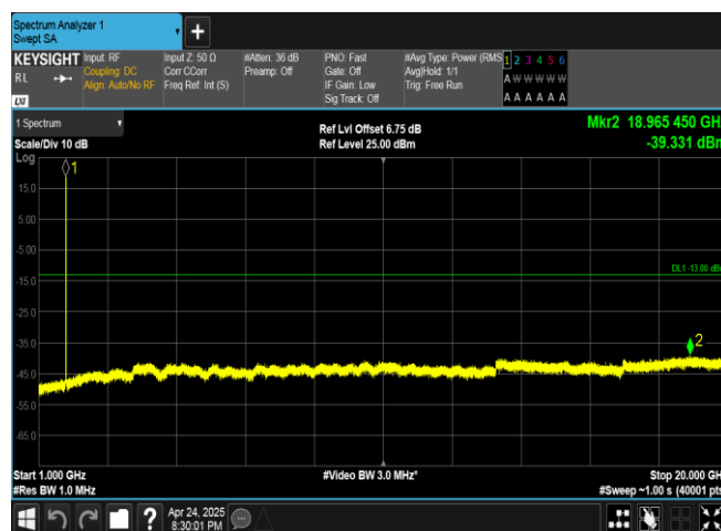
Band4-1513-1-1000~20000MHz-PASS
