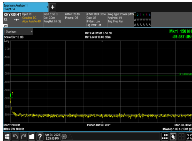
Band4-1513-1-0.15~30MHz-PASS
