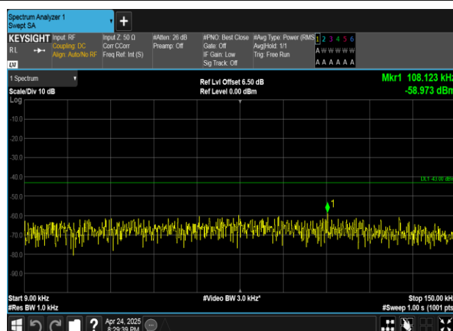
Band4-1513-1-0.009~0.15MHz-PASS
