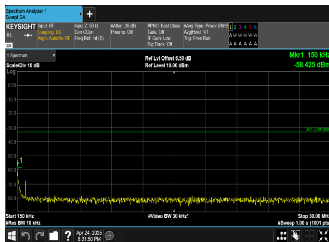
Band4-1513-2-0.15~30MHz-PASS
