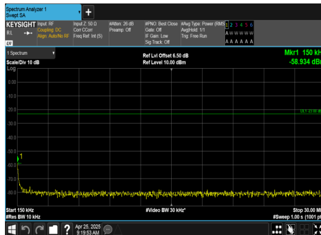
Band5-4233-1-0.15~30MHz-PASS
