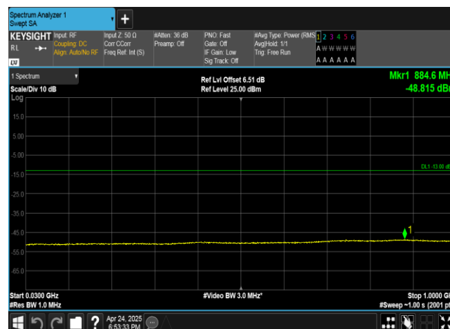
Band2-9400-4-30~1000MHz-PASS
