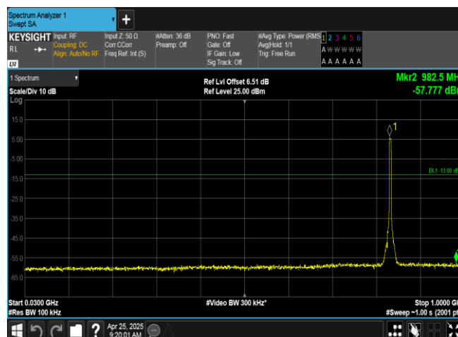
Band5-4233-1-30~1000MHz-PASS
