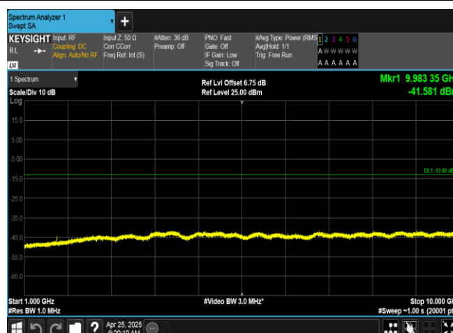
Band5-4233-1-1000~10000MHz-PASS
