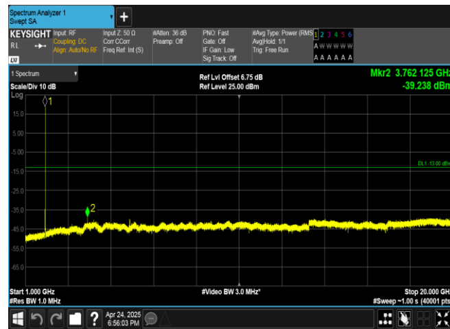
Band2-9400-5-1000~20000MHz-PASS
