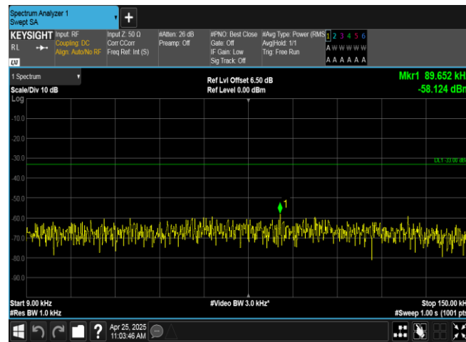
Band5-4182-5-0.009~0.15MHz-PASS
