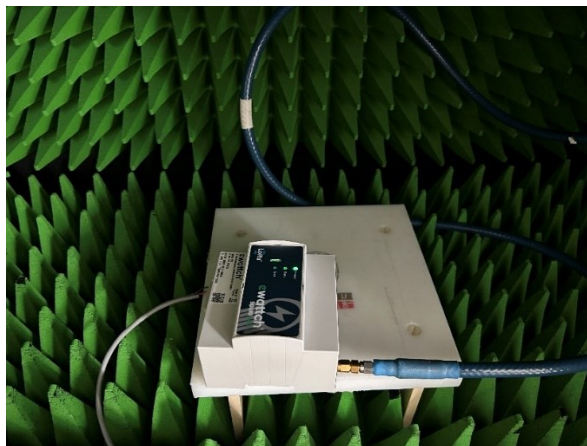
Photograph for Unwanted Emission into non-restricted frequency bands
