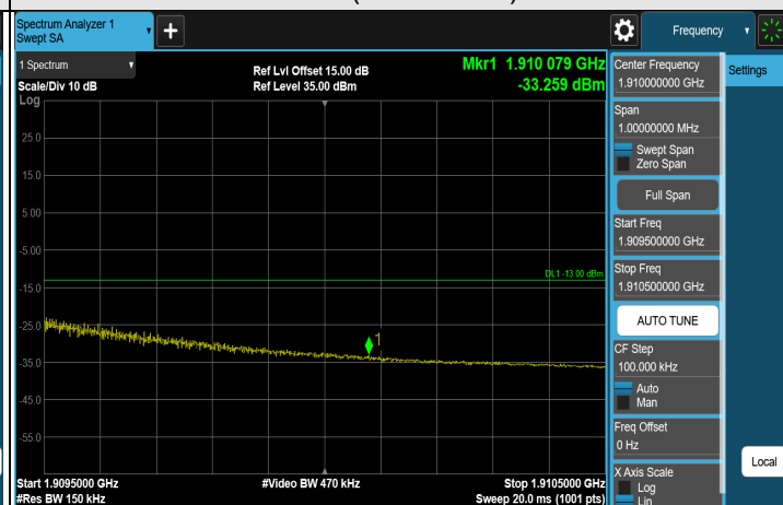
FULL (1902.5MHz)
