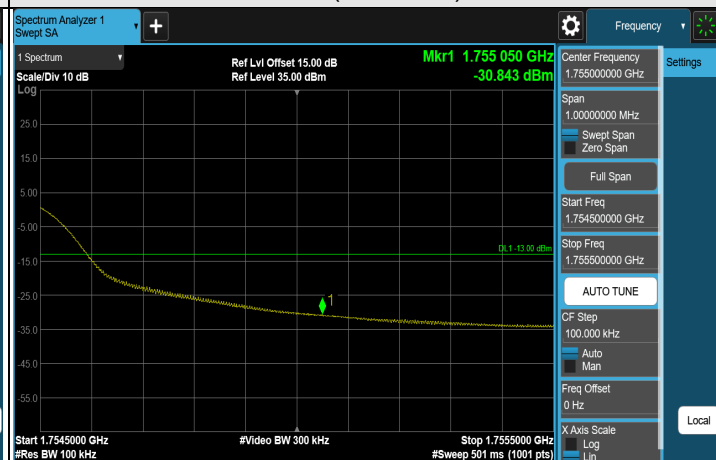
FULL (1750MHz)
