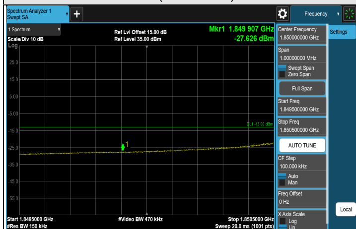
FULL (1857.5MHz)
