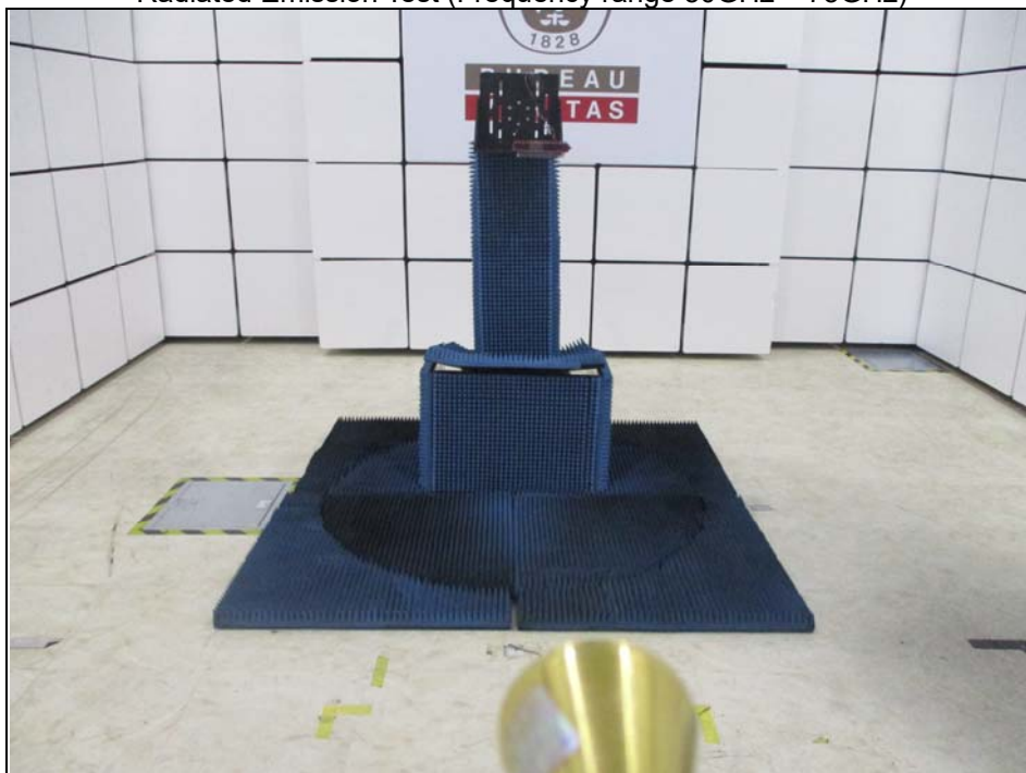
Radiated Emission Test (Frequency range 50GHz ~ 75GHz)
