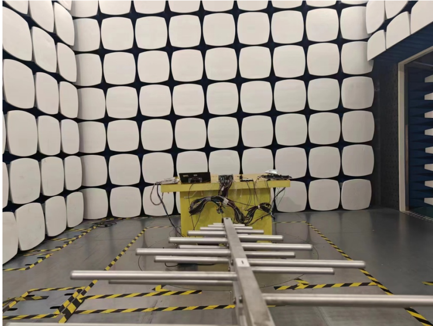
30MHz-1GHz
