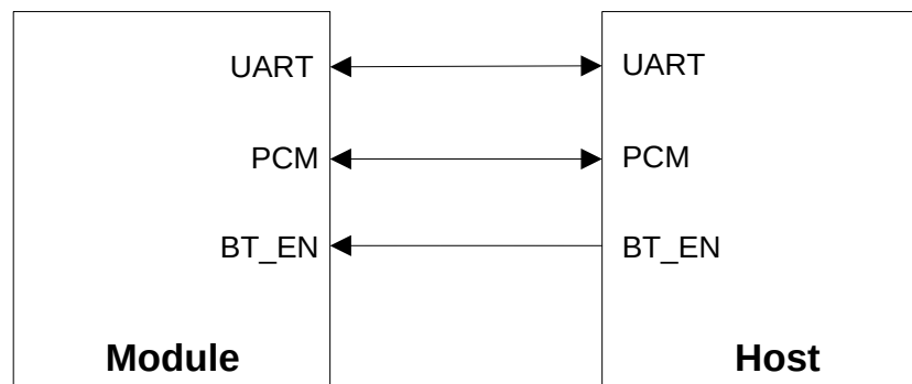
Figure 7: Block Diagram of Bluetooth Application Interface Connection
