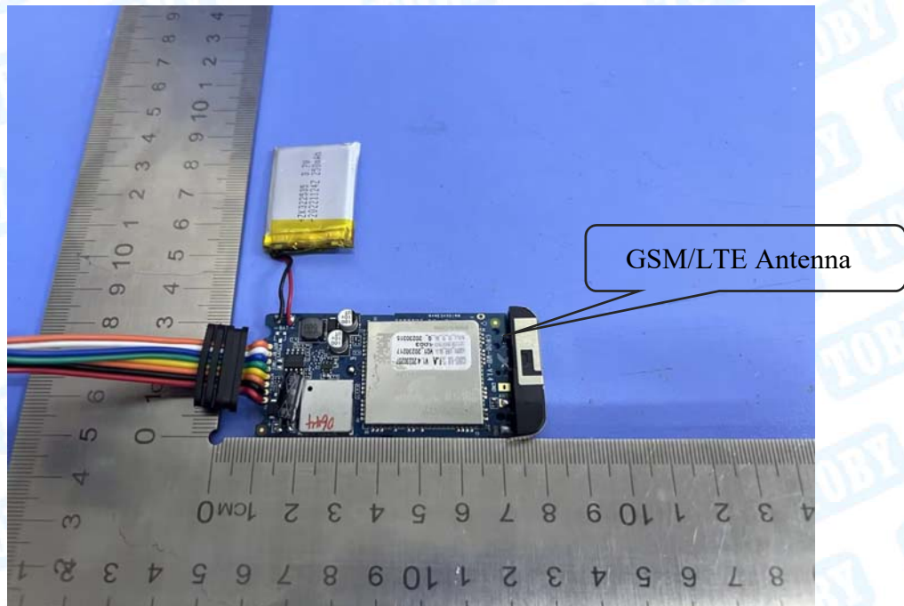
Photo 7 Appearance of PCB
