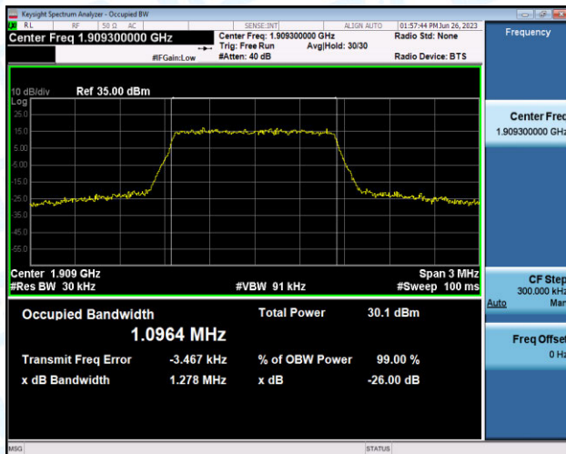
Band2-1.4MHz-QPSK-19193-6RB#0-PASS
