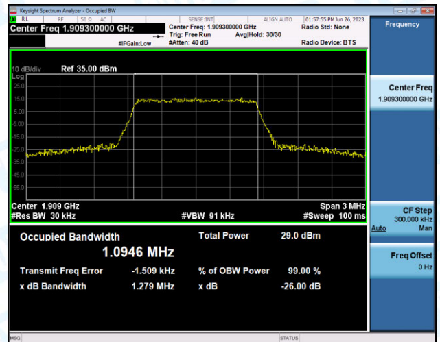
Band2-1.4MHz-16QAM-19193-6RB#0-PASS
