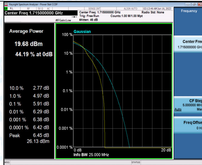
Band4-10MHz-16QAM-20000-27RB#0
