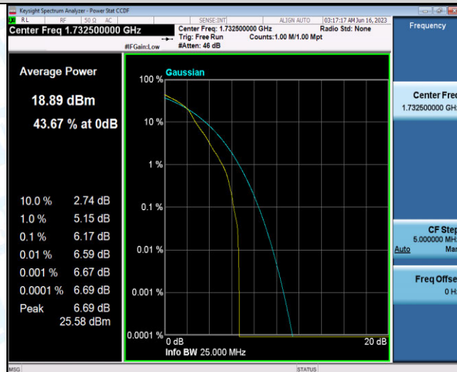
Band4-15MHz-16QAM-20175-27RB#0
