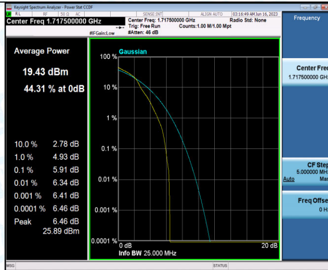
Band4-15MHz-16QAM-20025-27RB#0
