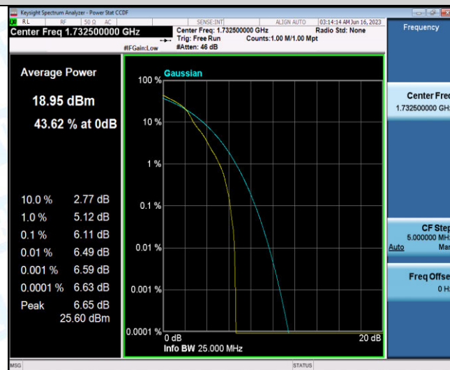
Band4-10MHz-16QAM-20175-27RB#0
