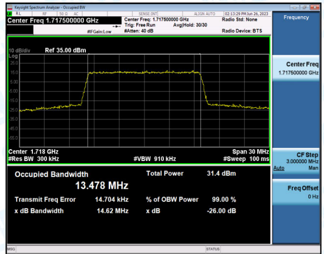
Band4-15MHz-QPSK-20325-75RB#0-PASS
