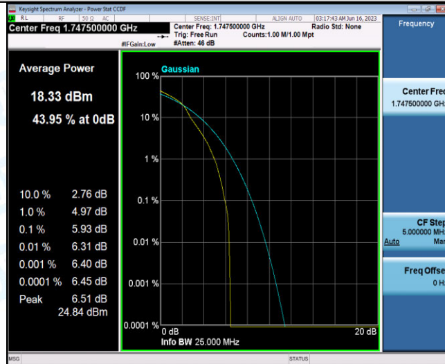
Band4-15MHz-16QAM-20325-27RB#0
