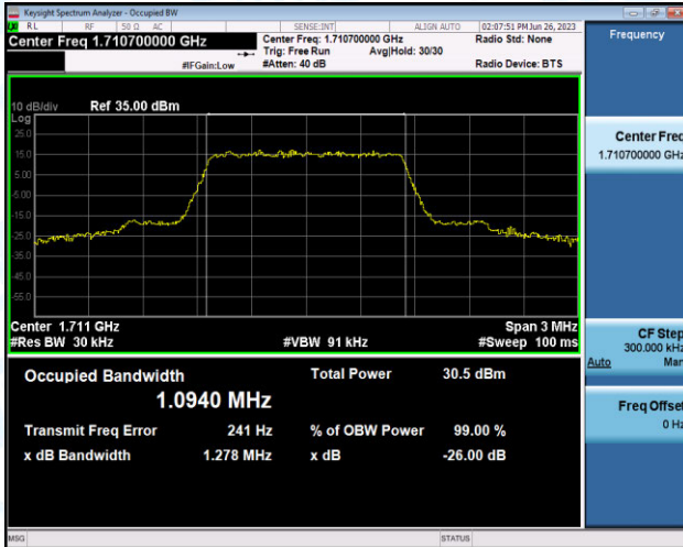
Band4-1.4MHz-QPSK-20175-6RB#0-PASS
