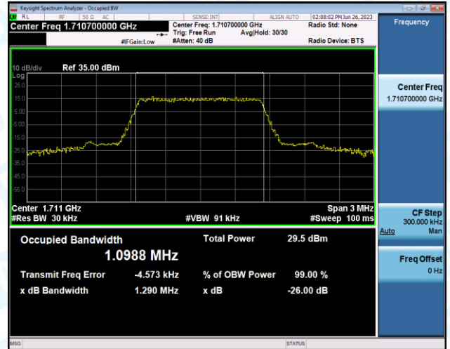
Band4-1.4MHz-16QAM-20175-6RB#0-PASS
