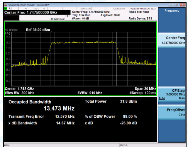
Band4-20MHz-QPSK-20175-100RB#0-PASS
