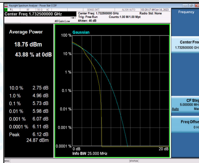
Band4-20MHz-16QAM-20175-27RB#0
