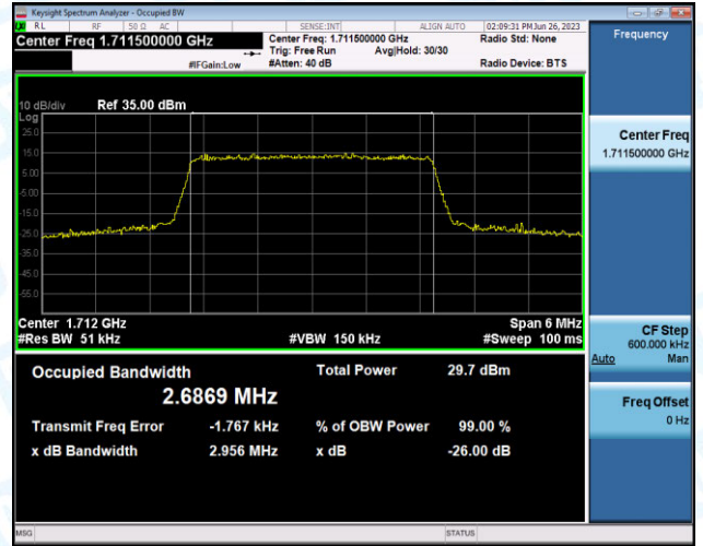
Band4-3MHz-16QAM-20175-15RB#0-PASS
