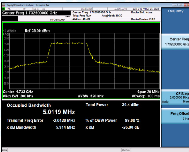
Band4-10MHz-16QAM-20175-27RB#0-PASS
