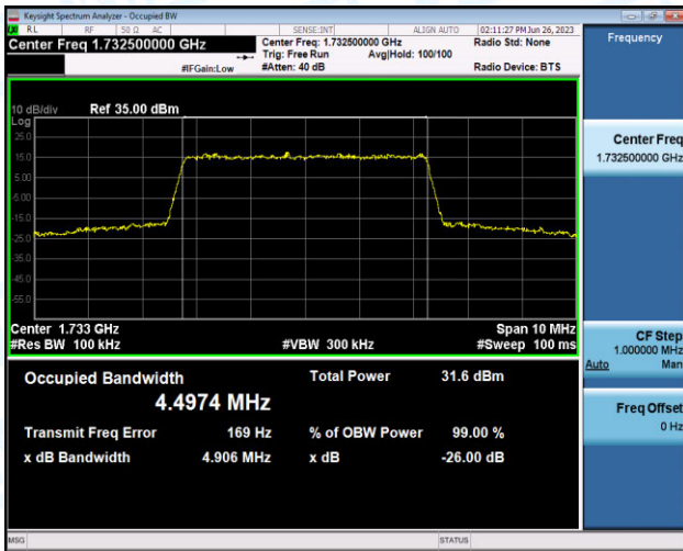
Band4-5MHz-QPSK-20375-25RB#0-PASS
