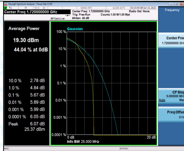
Band4-20MHz-16QAM-20050-27RB#0
