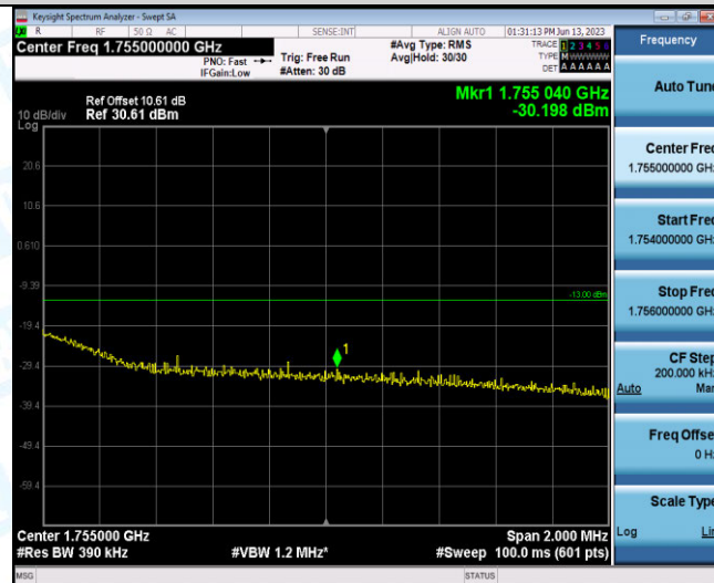
Band4-20MHz-16QAM-20300-27RB#0
