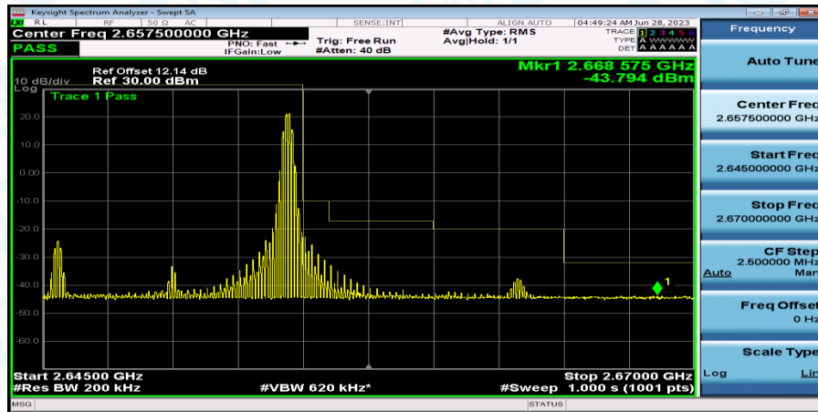
Band41_Band41_10MHz_QPSK_41190_1RB#49
