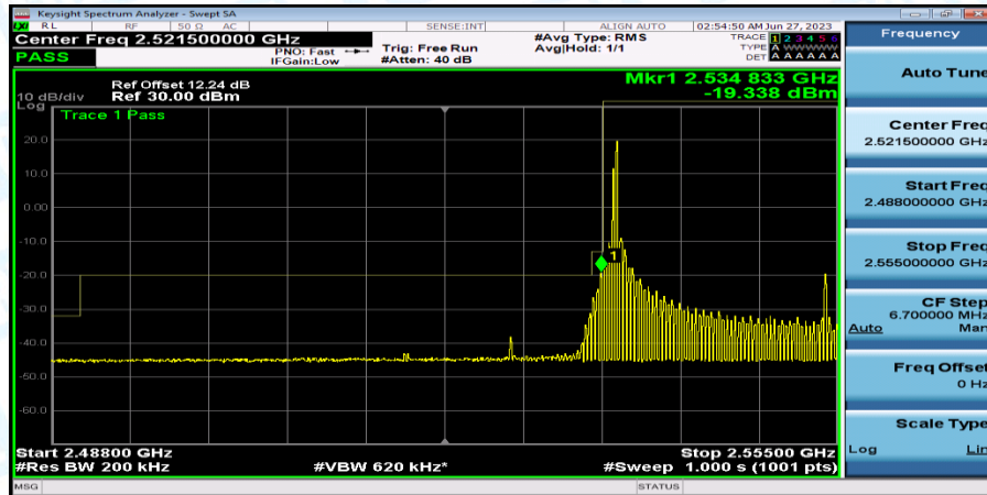
Band41_Band41_20MHz_16QAM_40140_1RB#0
