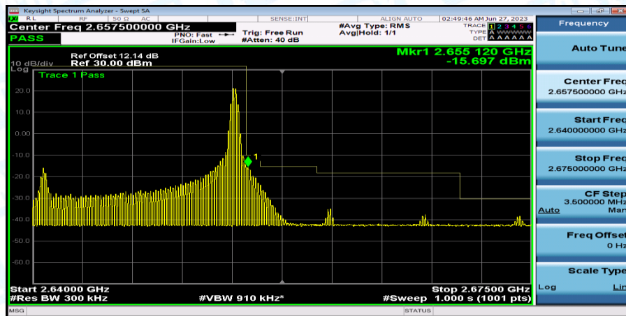
Band41_Band41_15MHz_QPSK_41165_1RB#74
