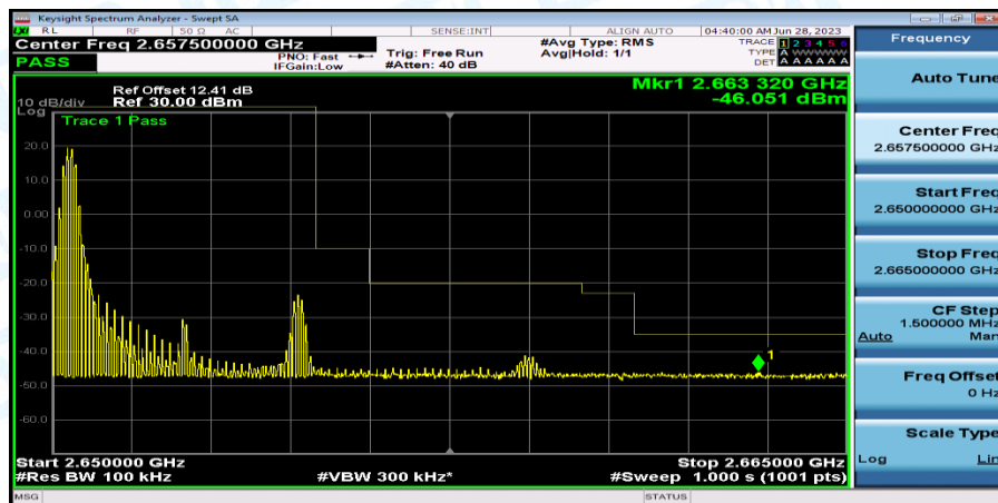
Band41_Band41_5MHz_16QAM_41215_1RB#0
