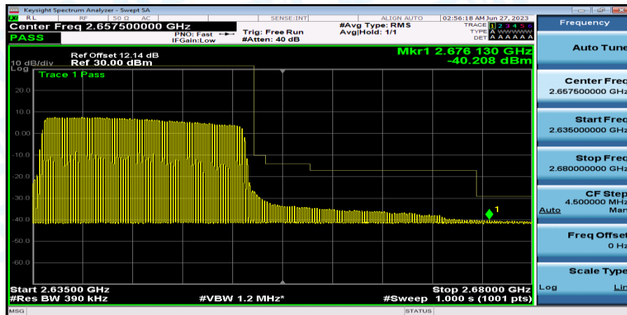
Band41_Band41_20MHz_QPSK_41140_100RB#0
