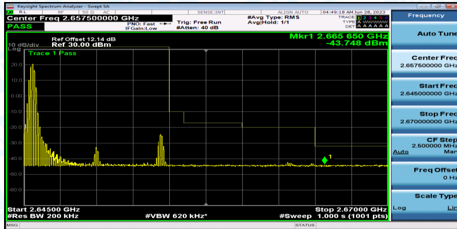
Band41_Band41_10MHz_16QAM_41190_1RB#0
