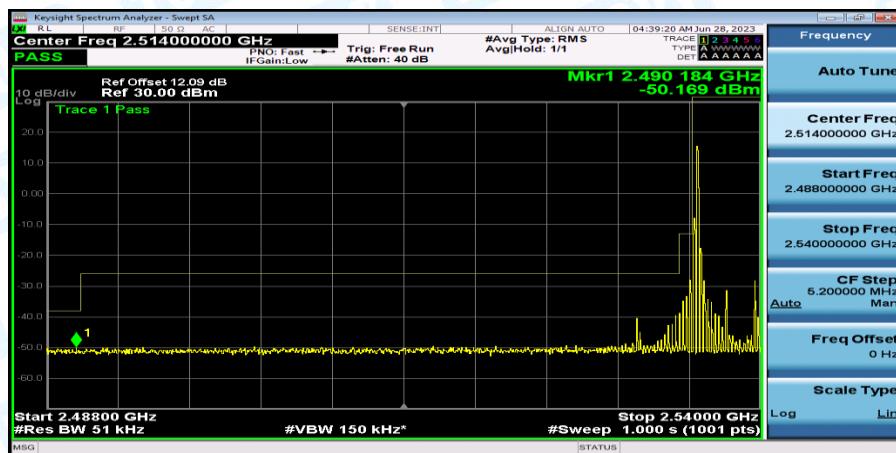
Band41_Band41_5MHz_16QAM_40065_1RB#0
