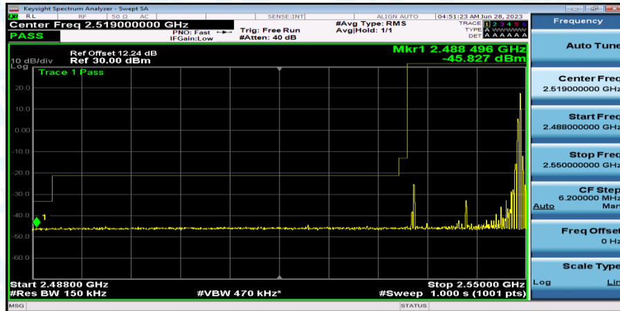
Band41_Band41_15MHz_16QAM_40115_1RB#74
