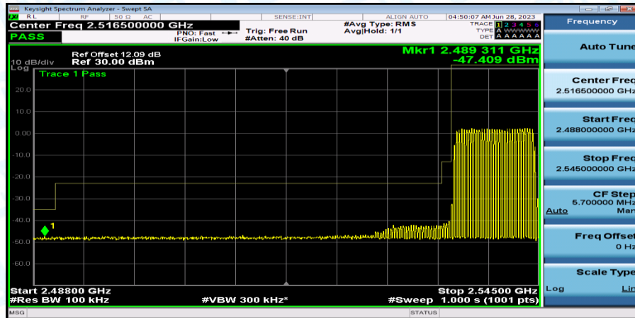
Band41_Band41_10MHz_QPSK_40090_50RB#0
