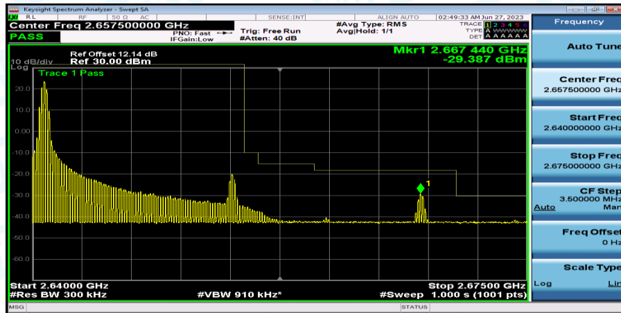
Band41_Band41_15MHz_QPSK_41165_1RB#0
