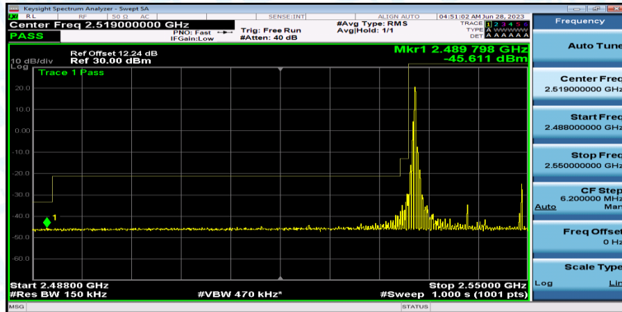
Band41_Band41_15MHz_QPSK_40115_1RB#0
