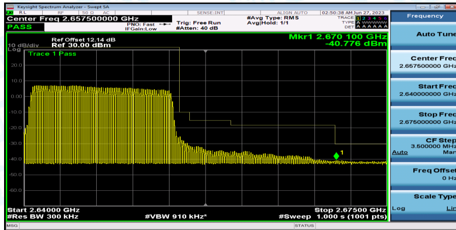
Band41_Band41_15MHz_QPSK_41165_75RB#0
