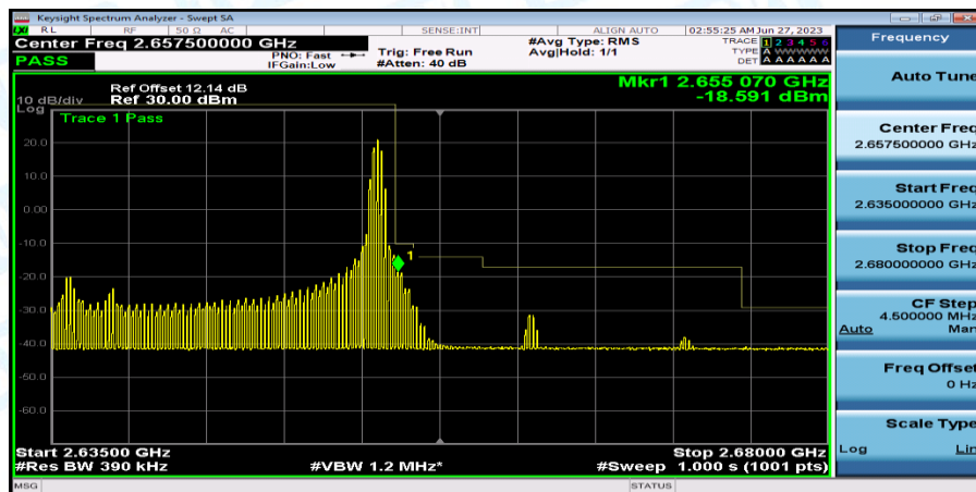
Band41_Band41_20MHz_QPSK_41140_1RB#99
