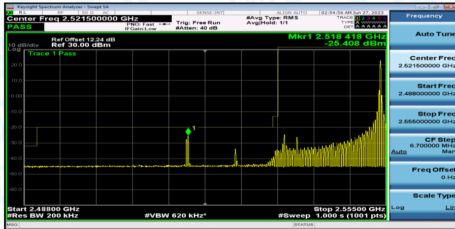
Band41_Band41_20MHz_QPSK_40140_1RB#99
