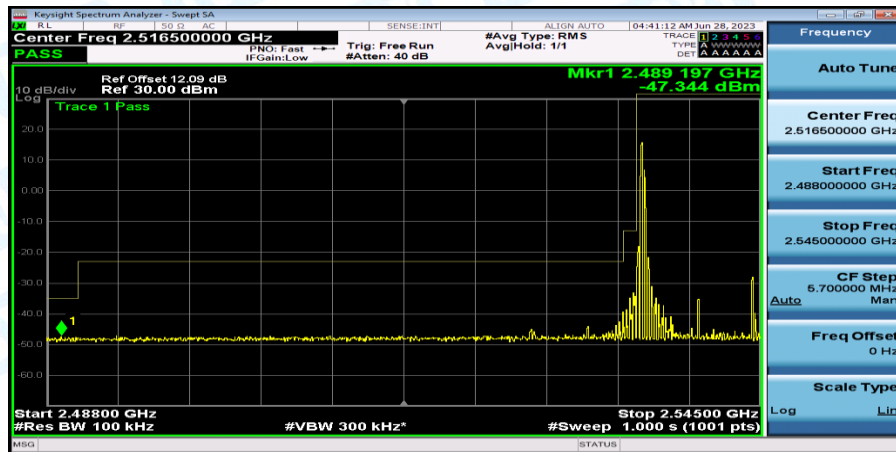
Band41_Band41_10MHz_16QAM_40090_1RB#0
