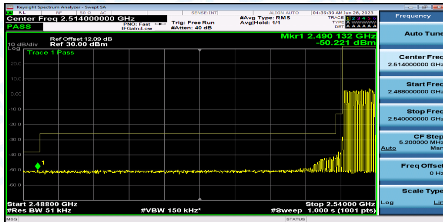
Band41_Band41_5MHz_QPSK_40065_25RB#0
