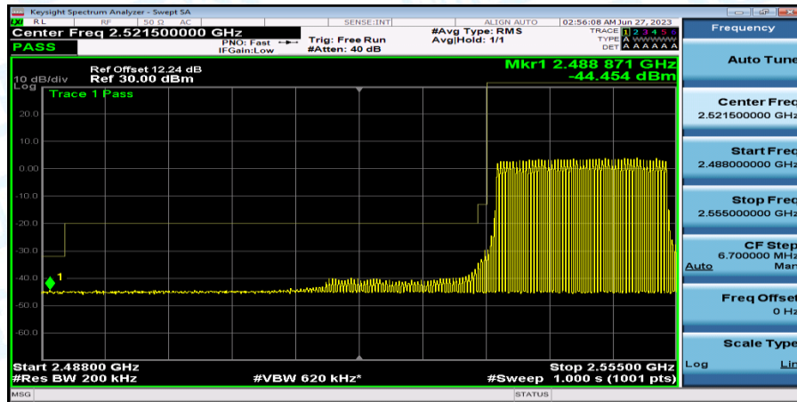
Band41_Band41_20MHz_QPSK_40140_100RB#0
