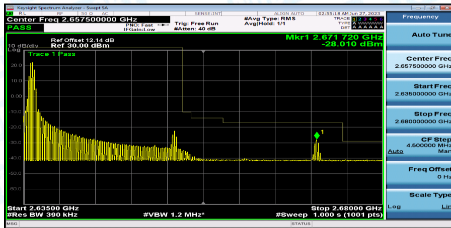
Band41_Band41_20MHz_16QAM_41140_1RB#0
