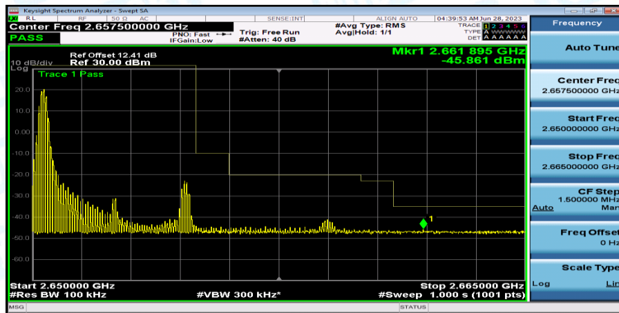
Band41_Band41_5MHz_QPSK_41215_1RB#0
