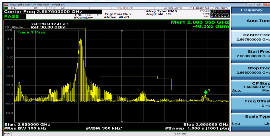
Band41_Band41_5MHz_QPSK_41215_1RB#24
