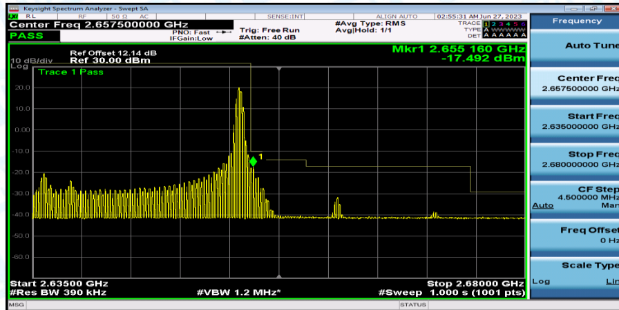
Band41_Band41_20MHz_16QAM_41140_1RB#99
