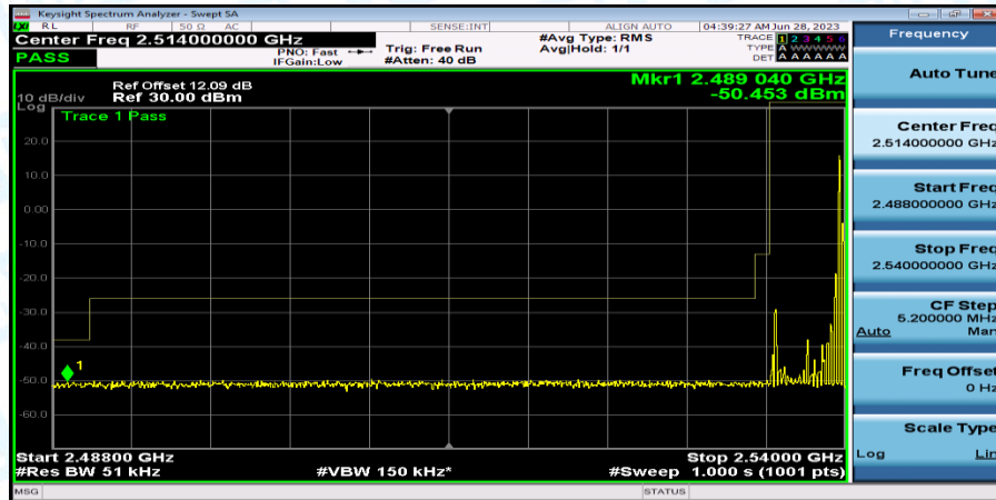
Band41_Band41_5MHz_QPSK_40065_1RB#24
