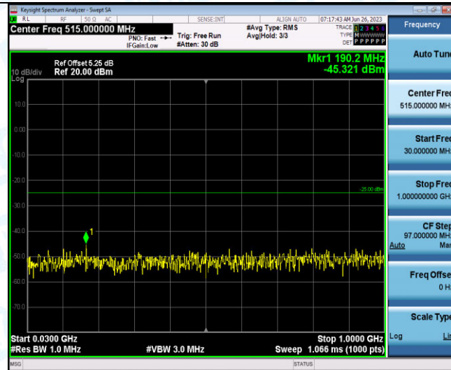
Band41-5MHz-QPSK-41215-1RB#0-Range3:30~1000MHz
