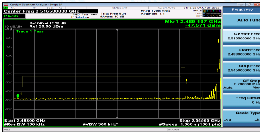
Band41_Band41_10MHz_16QAM_40090_1RB#49
