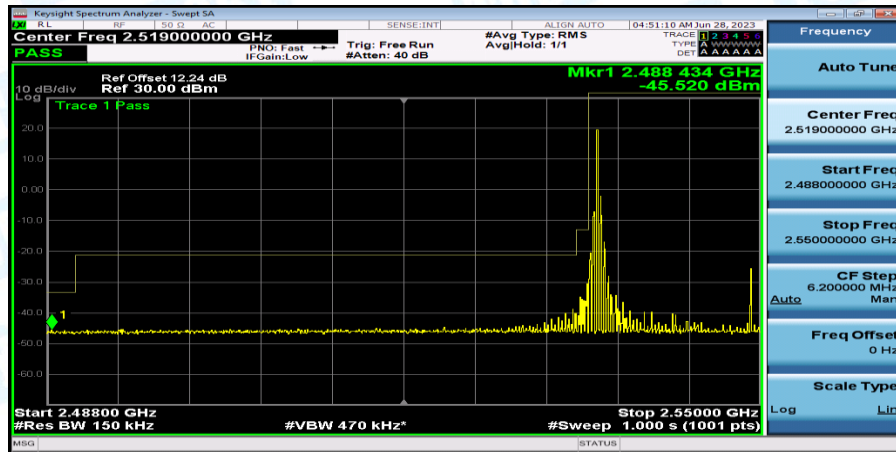
Band41_Band41_15MHz_16QAM_40115_1RB#0
