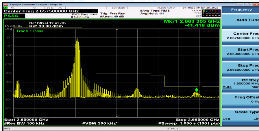
Band41_Band41_5MHz_16QAM_41215_1RB#24
