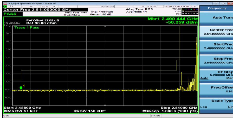
Band41_Band41_5MHz_16QAM_40065_1RB#24
