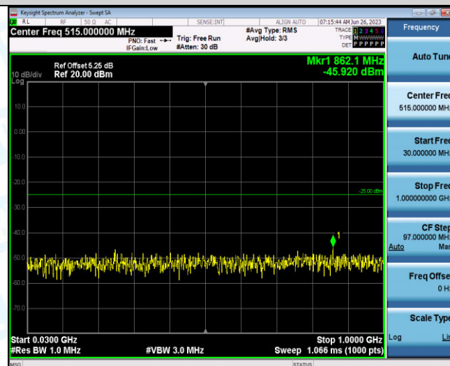
Band41-5MHz-QPSK-40640-1RB#0-Range3:30~1000MHz
