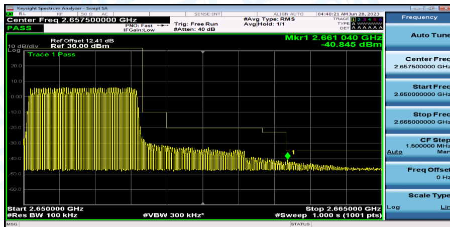
Band41_Band41_5MHz_QPSK_41215_25RB#0
