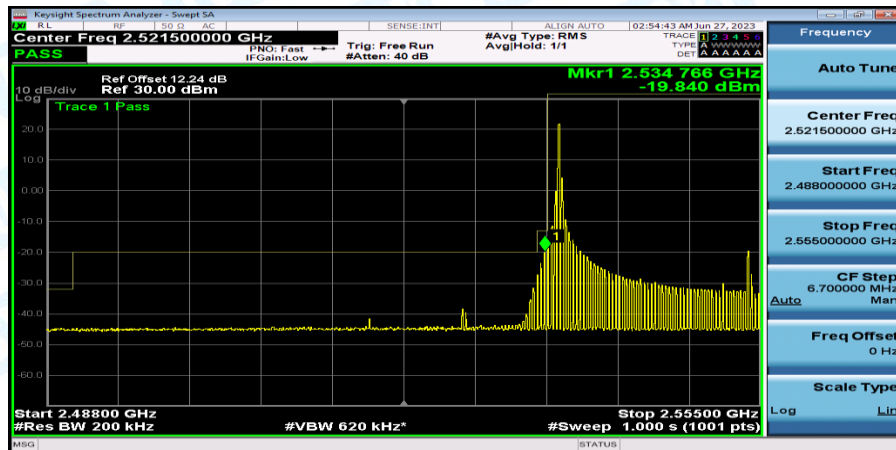
Band41_Band41_20MHz_QPSK_40140_1RB#0
