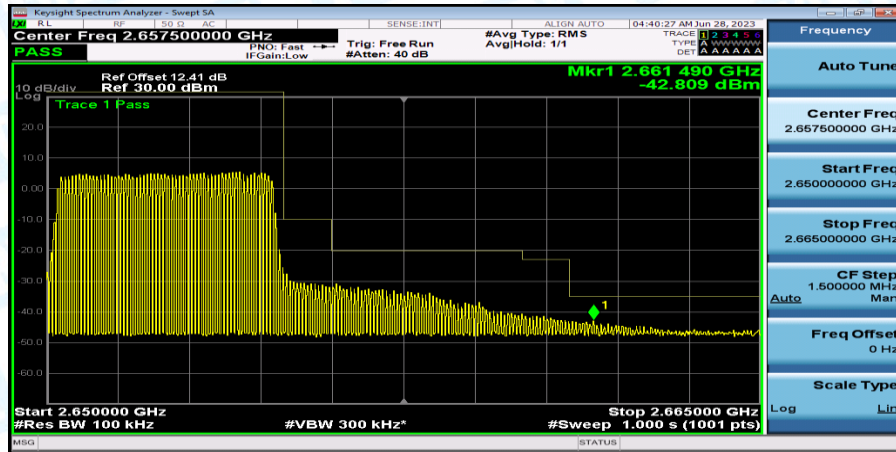
Band41_Band41_5MHz_16QAM_41215_25RB#0
