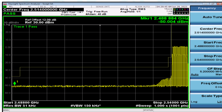
Band41_Band41_5MHz_16QAM_40065_25RB#0
