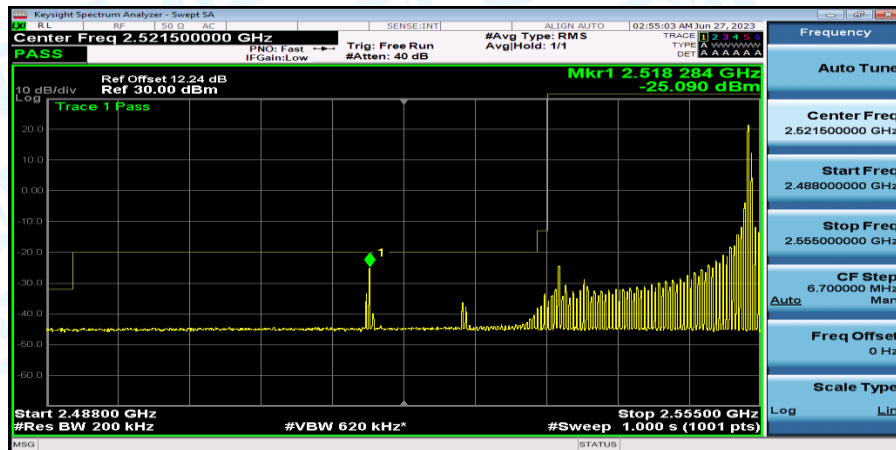
Band41_Band41_20MHz_16QAM_40140_1RB#99
