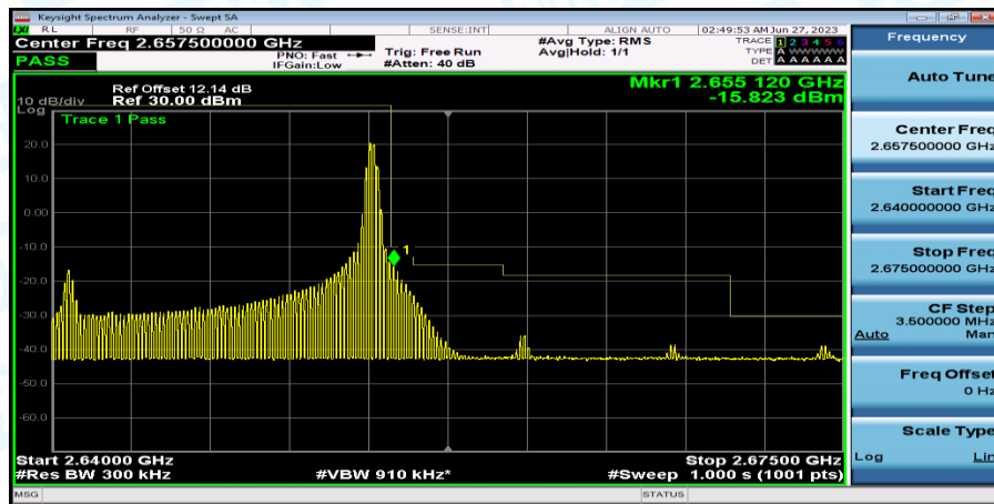
Band41_Band41_15MHz_16QAM_41165_1RB#74
