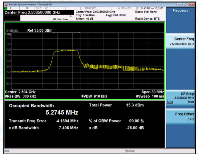
Band41-15MHz-16QAM-41515-27RB#0-PASS
