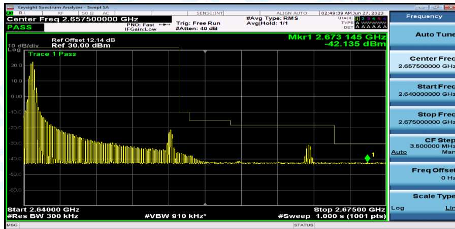
Band41_Band41_15MHz_16QAM_41165_1RB#0
