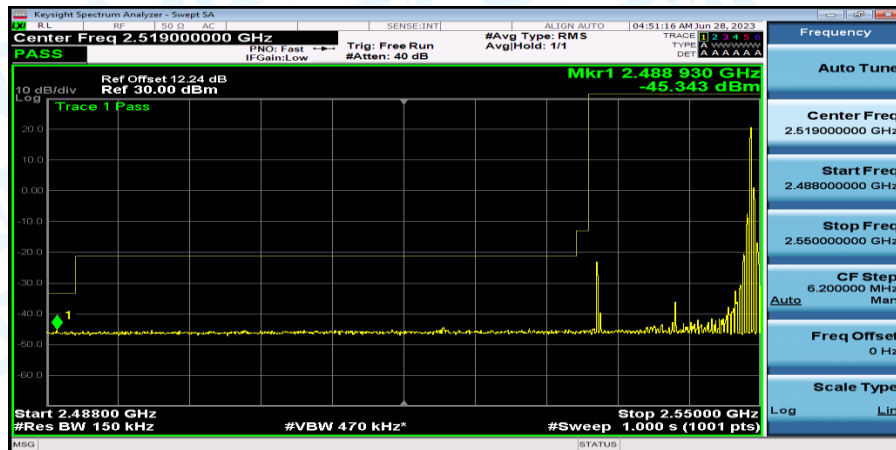
Band41_Band41_15MHz_QPSK_40115_1RB#74
