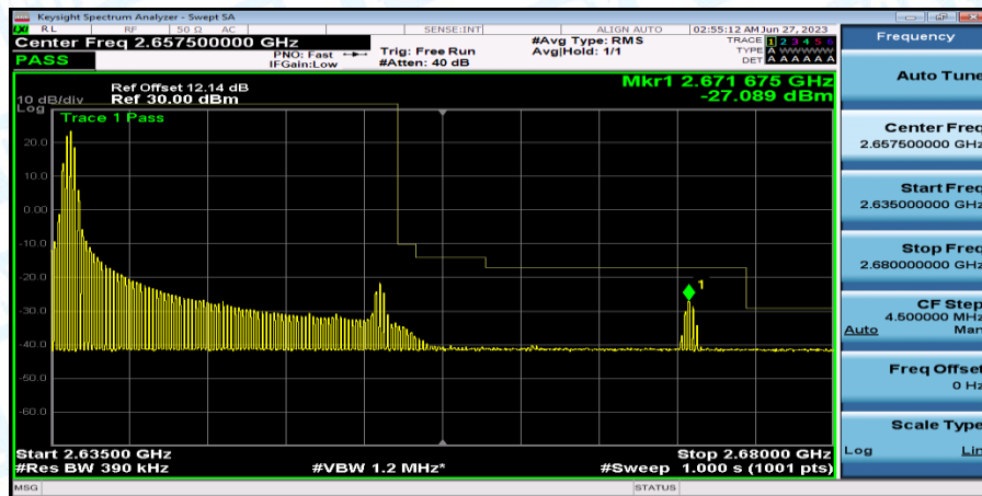
Band41_Band41_20MHz_QPSK_41140_1RB#0
