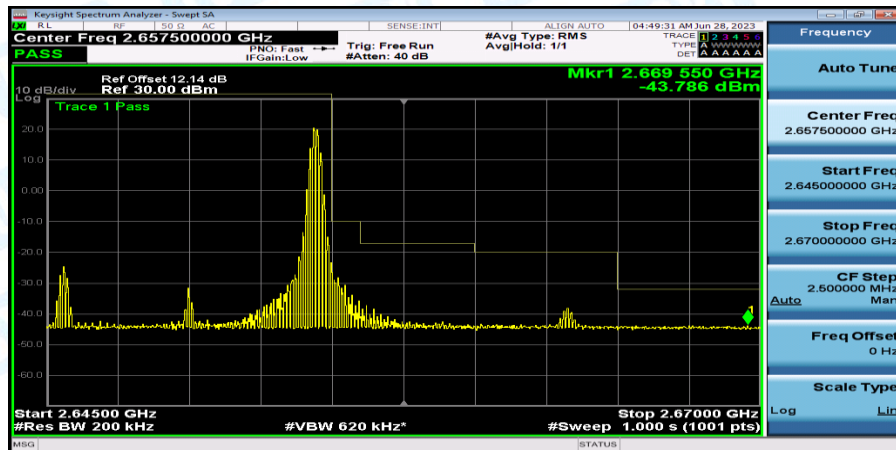
Band41_Band41_10MHz_16QAM_41190_1RB#49
