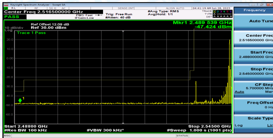
Band41_Band41_10MHz_QPSK_40090_1RB#49
