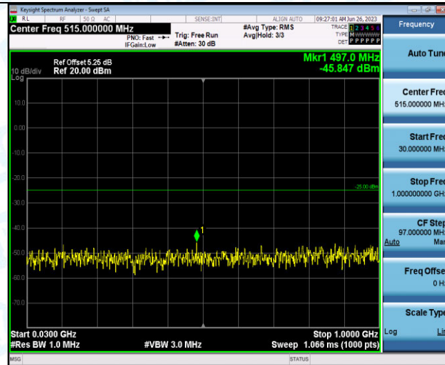
Band41-10MHz-16QAM-41190-1RB#0-Range3:30~1000MHz
