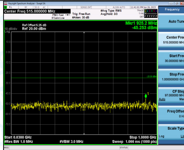
Band41-15MHz-QPSK-41165-1RB#0-Range3:30~1000MHz
