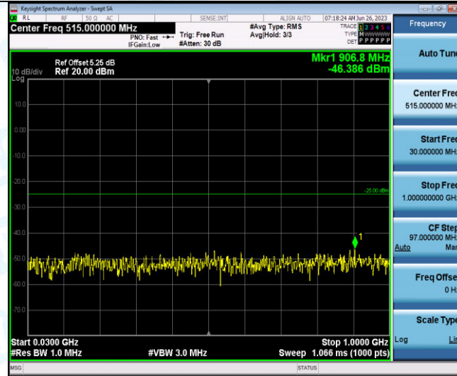
Band41-5MHz-16QAM-41215-1RB#0-Range3:30~1000MHz
