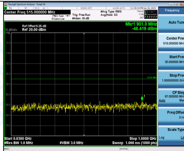
Band41-15MHz-16QAM-40115-1RB#0-Range1:30~1000MHz
