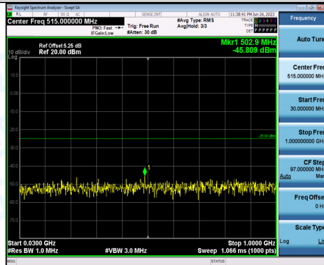
Band41-15MHz-QPSK-40115-1RB#0-Range1:30~1000MHz
