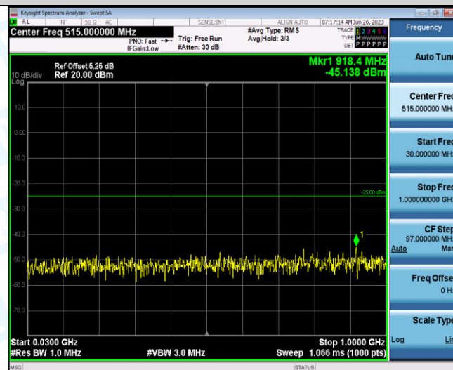
Band41-5MHz-16QAM-40640-1RB#0-Range1:30~1000MHz
