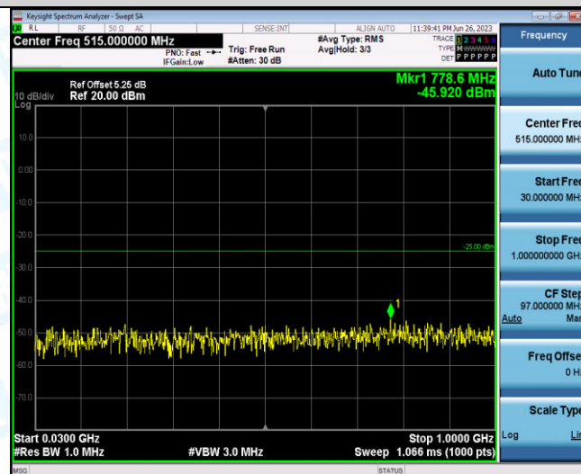
Band41-15MHz-QPSK-40640-1RB#0-Range3:30~1000MHz
