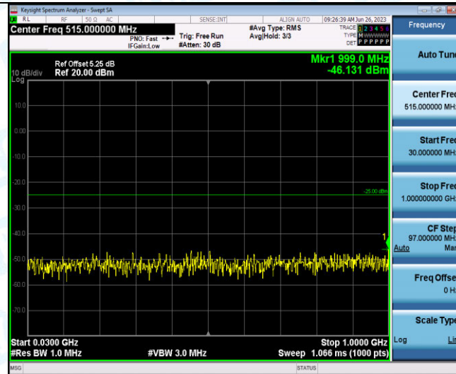
Band41-10MHz-QPSK-41190-1RB#0-Range1:30~1000MHz
