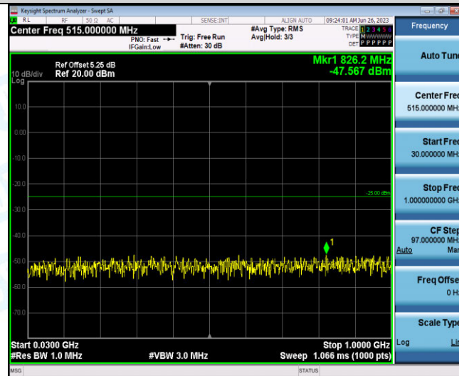
Band41-10MHz-QPSK-40090-1RB#0-Range1:30~1000MHz
