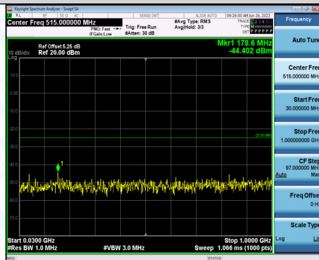
Band41-10MHz-16QAM-40640-1RB#0-Range1:30~1000MHz
