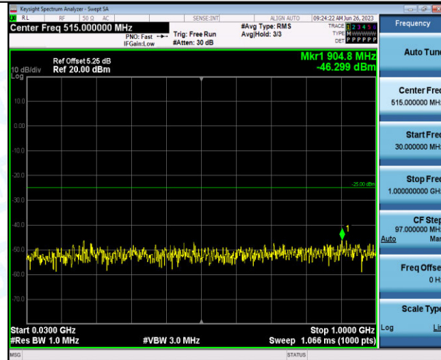
Band41-10MHz-16QAM-40090-1RB#0-Range3:30~1000MHz
