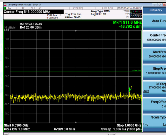
Band41-10MHz-QPSK-40640-1RB#0-Range3:30~1000MHz
