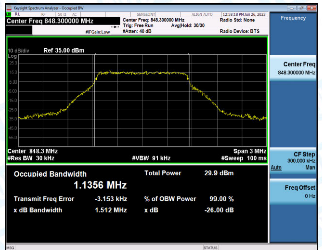
Band5-1.4MHz-16QAM-20643-6RB#0-PASS
