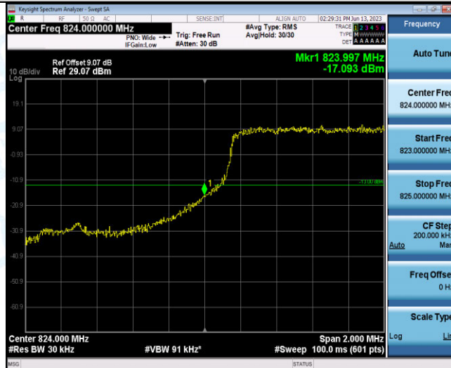
Band5-1.4MHz-QPSK-20643-6RB#0
