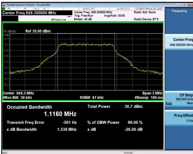
Band5-1.4MHz-QPSK-20643-6RB#0-PASS
