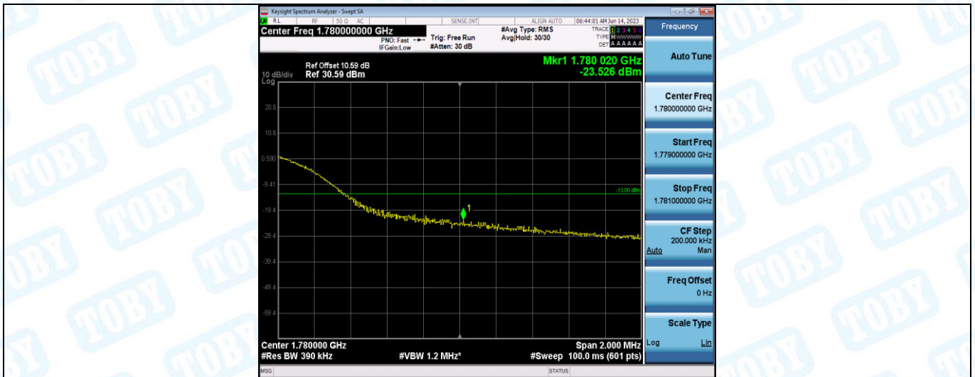
Band66-20MHz-16QAM-132072-27RB#0
