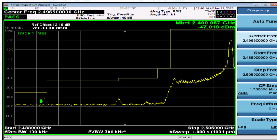
Band7_5MHz_16QAM_20775_1RB#24
