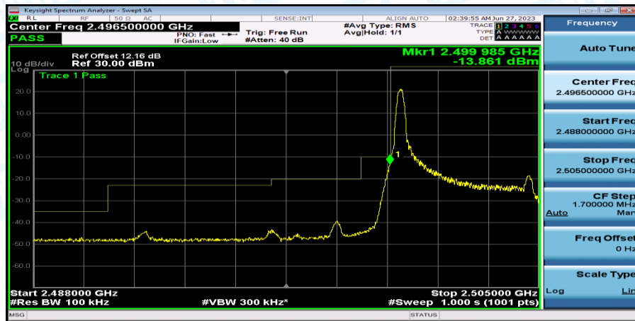
Band7_5MHz_QPSK_20775_1RB#0
