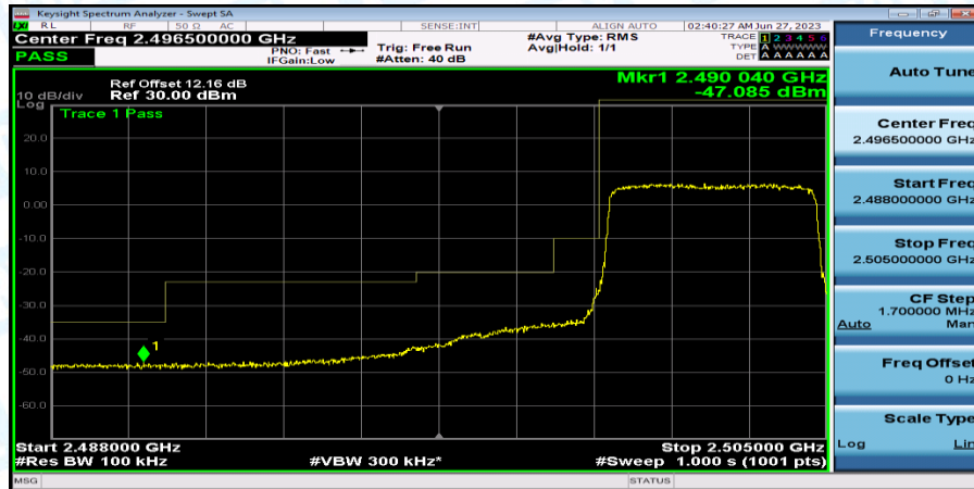
Band7_5MHz_16QAM_20775_25RB#0
