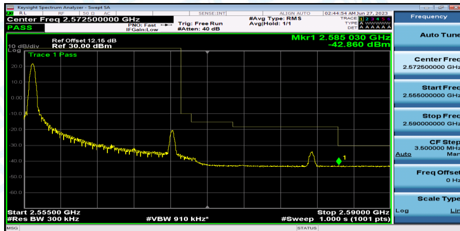
Band7_15MHz_16QAM_21375_1RB#0
