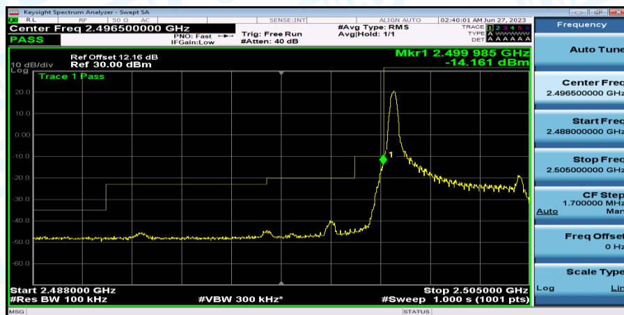
Band7_5MHz_16QAM_20775_1RB#0
