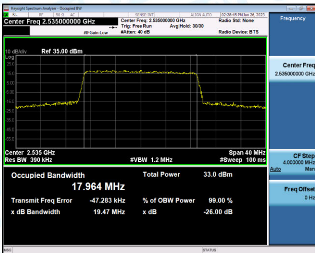
Band7-20MHz-QPSK-21100-100RB#0-PASS
