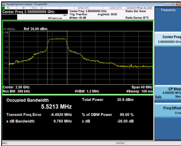
Band7-15MHz-QPSK-21100-75RB#0-PASS
