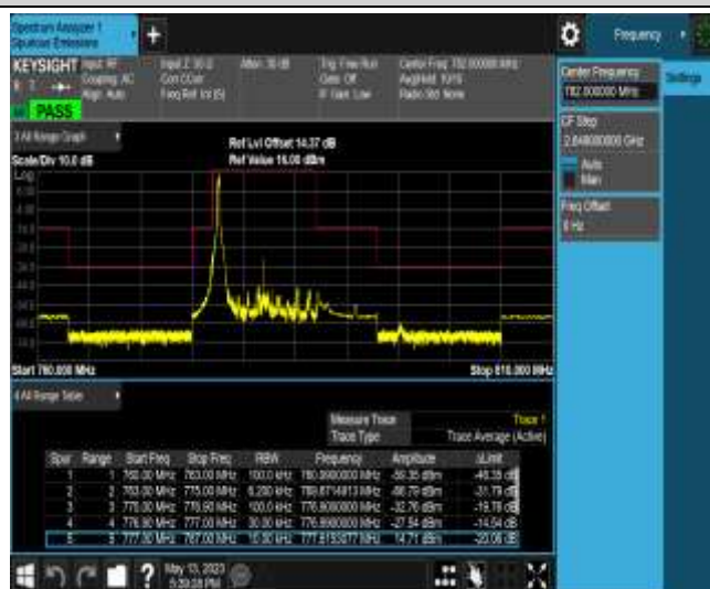
Band13-10MHz-QPSK-23230-1RB#0
