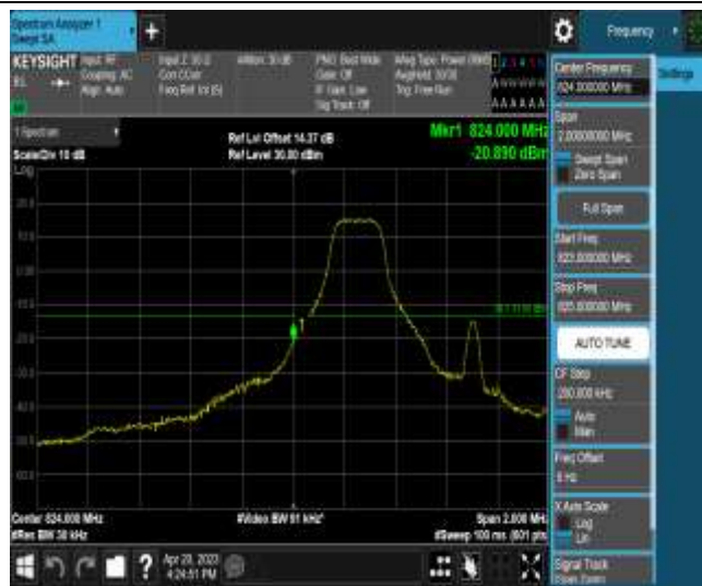
Band5-1.4MHz-QPSK-20407-1RB#0
