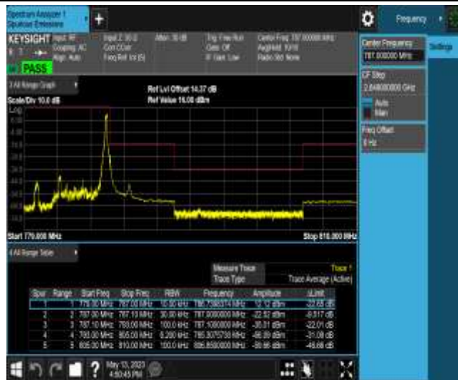
Band13-5MHz-16QAM-23255-1RB#24
