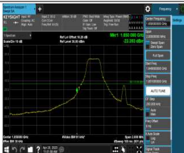
Band2-1.4MHz-16QAM-18607-1RB#0
