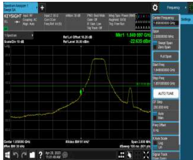
Band2-1.4MHz-QPSK-18607-1RB#0
