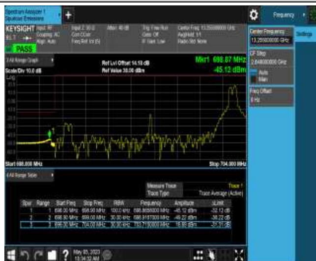
Band12-5MHz-QPSK-23035-1RB#24--45.12-32.12
