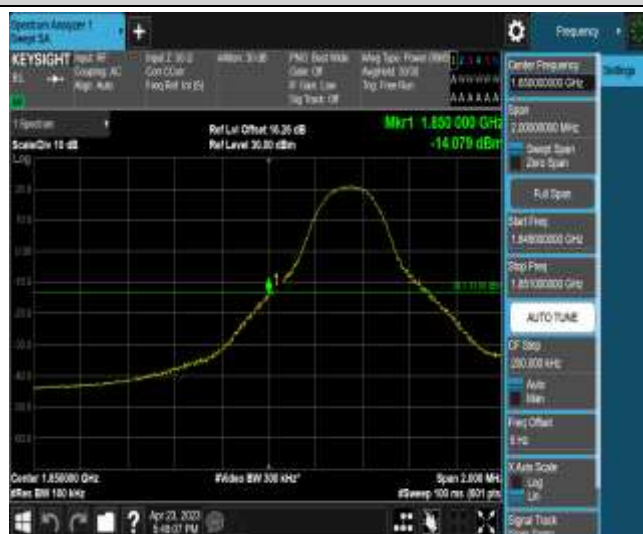
Band25-5MHz-16QAM-26065-1RB#0
