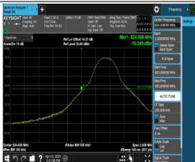
Band26-5MHz-16QAM-26815-1RB#0
