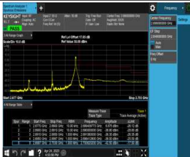
Band41-10MHz-QPSK-41540-1RB#49
