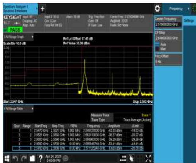
Band38-20MHz-16QAM-37850-1RB#0
