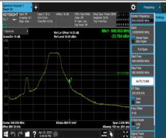
Band26-1.4MHz-16QAM-27033-1RB#5
