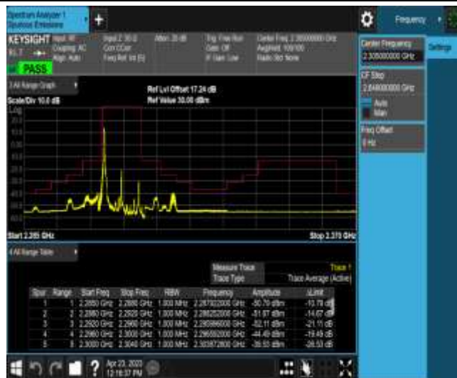
Band40-10MHz-16QAM-38750-1RB#0
