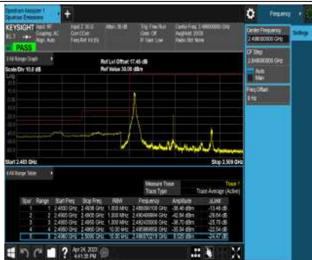
Band41-10MHz-16QAM-39700-1RB#0
