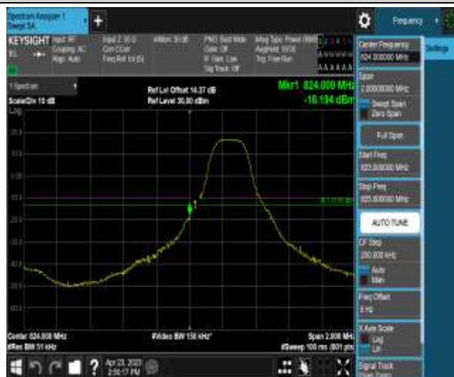
Band26-3MHz-QPSK-26805-1RB#0
