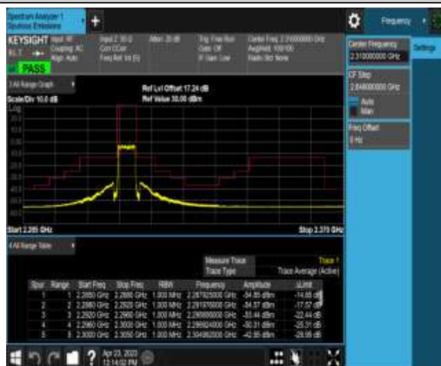
Band40-5MHz-16QAM-38775-25RB#0
