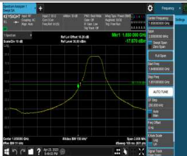
Band25-3MHz-16QAM-26055-1RB#0
