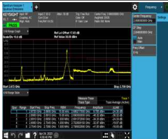
Band41-15MHz-QPSK-41515-1RB#74
