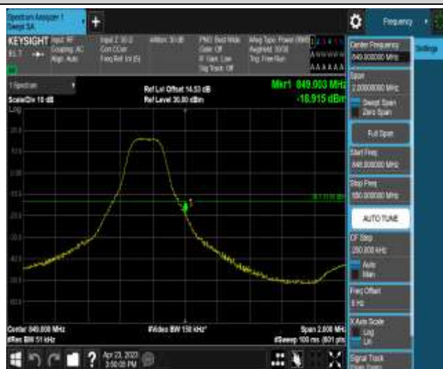
Band26-3MHz-16QAM-27025-1RB#14
