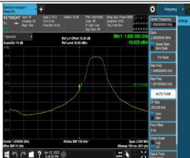
Band25-3MHz-QPSK-26055-1RB#0
