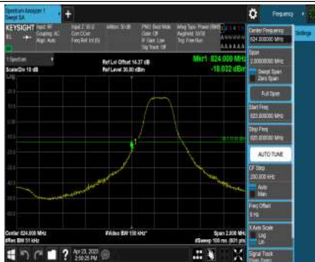
Band26-3MHz-16QAM-26805-1RB#0
