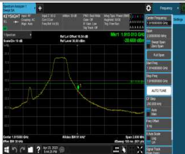
Band25-1.4MHz-16QAM-26683-1RB#5
