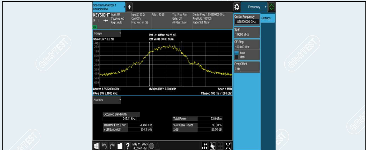
PCS1900-512
