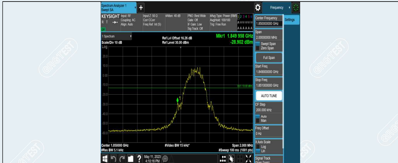
PCS1900-512
