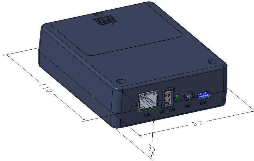
Figure 2: Equipment size drawing
