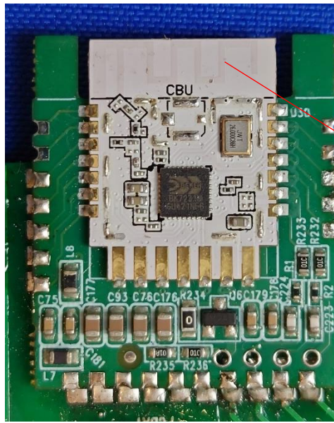
BLE+2.4G WiFi Antenna
