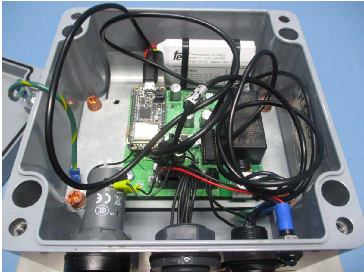
INTERNAL LAYOUT
