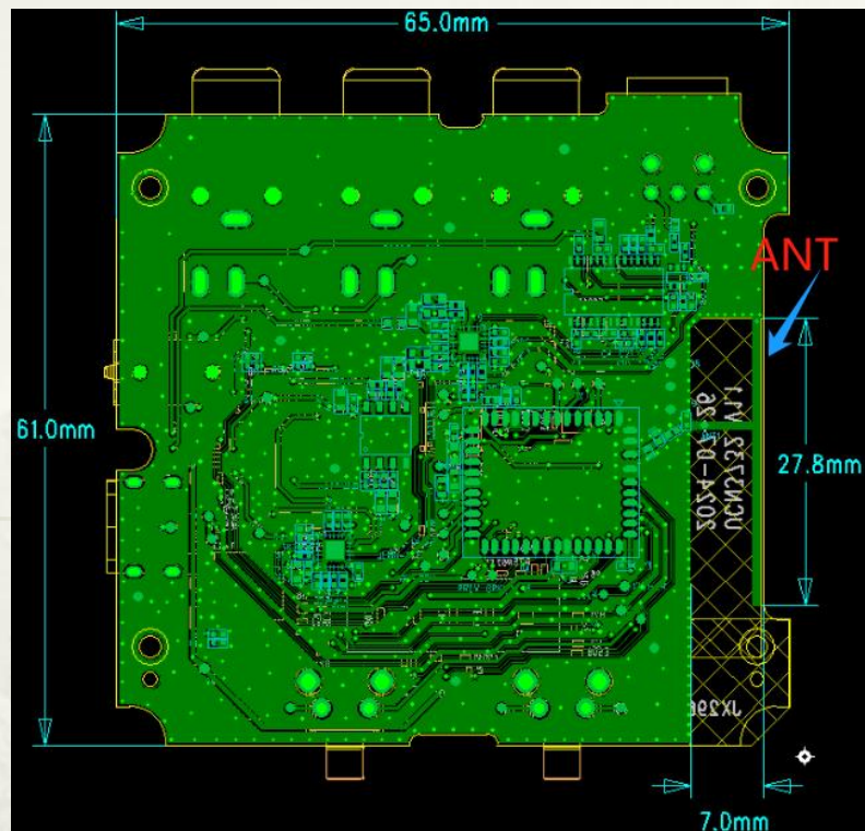
Antenna type: ANT-10 dimensions: L27.8*W7mm
