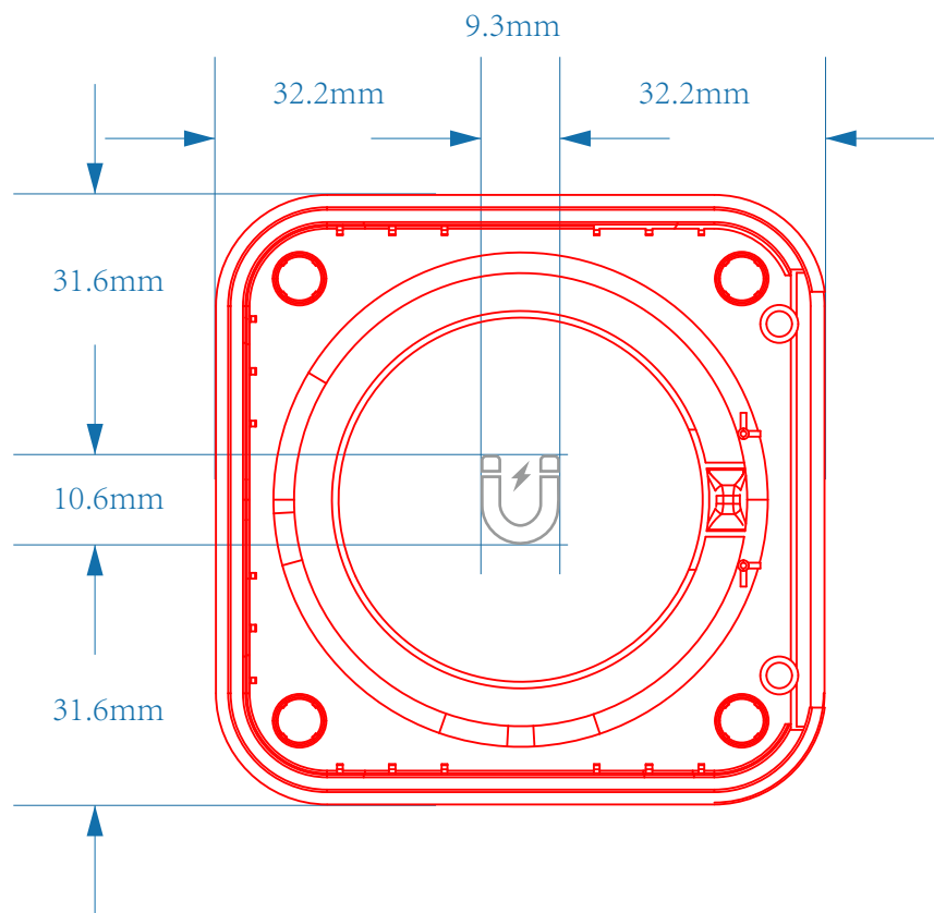
Magnetic suction phone upper case
