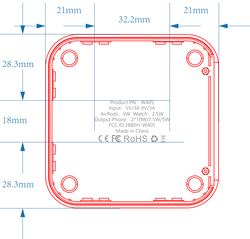
Non magnetic suction phone case
