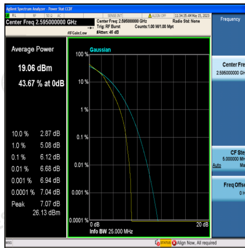
Band38-10MHz-16QAM-38000-50RB#0
