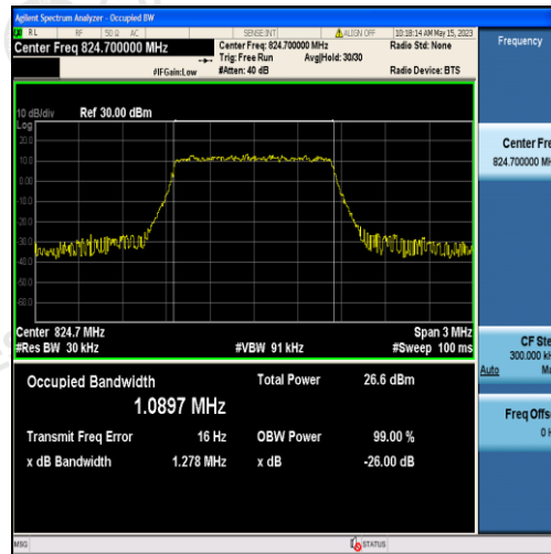
Band5-1.4MHz-QPSK-20407-6RB#0-1.0897
