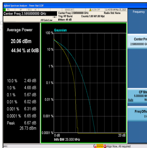
Band38-15MHz-QPSK-38000-75RB#0
