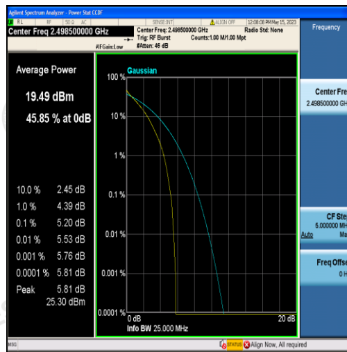
Band41-5MHz-QPSK-39675-25RB#0
