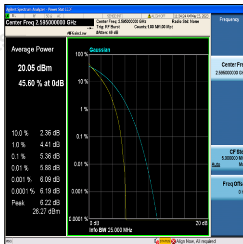
Band38-10MHz-QPSK-38000-50RB#0
