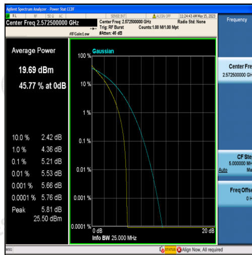
Band38-5MHz-QPSK-37775-25RB#0
