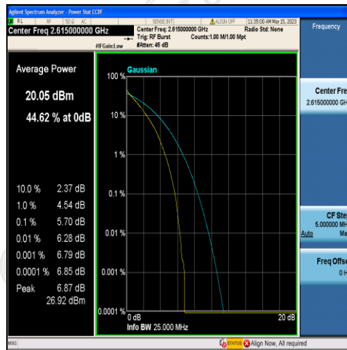
Band38-10MHz-QPSK-38200-50RB#0
