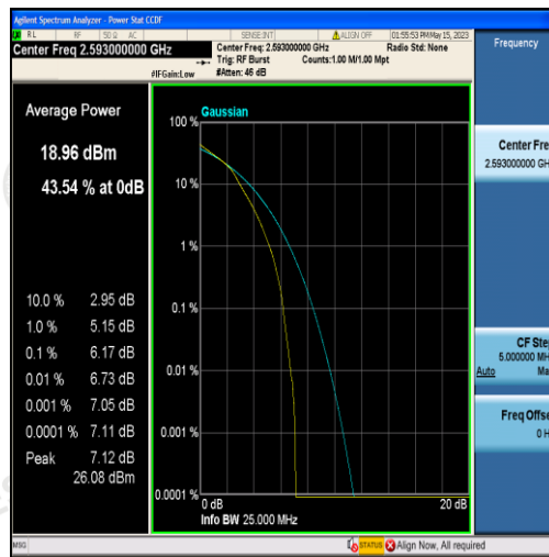
Band41-15MHz-16QAM-40620-75RB#0
