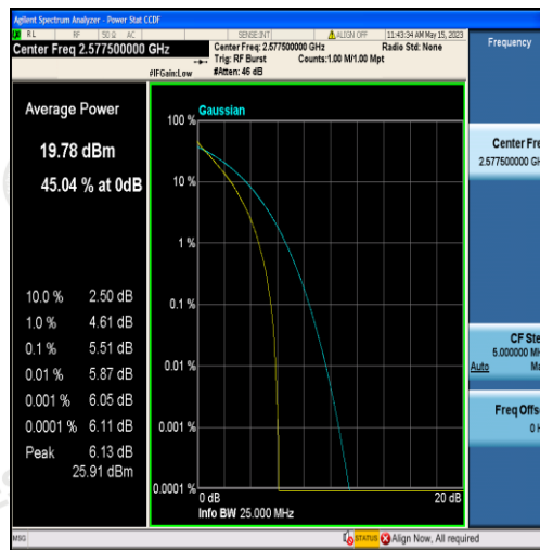
Band38-15MHz-QPSK-37825-75RB#0
