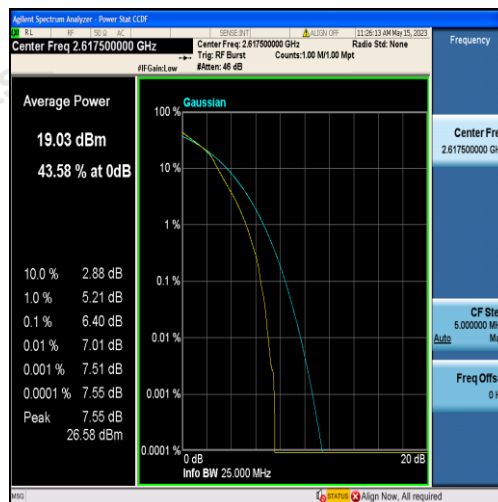
Band38-5MHz-16QAM-38225-25RB#0
