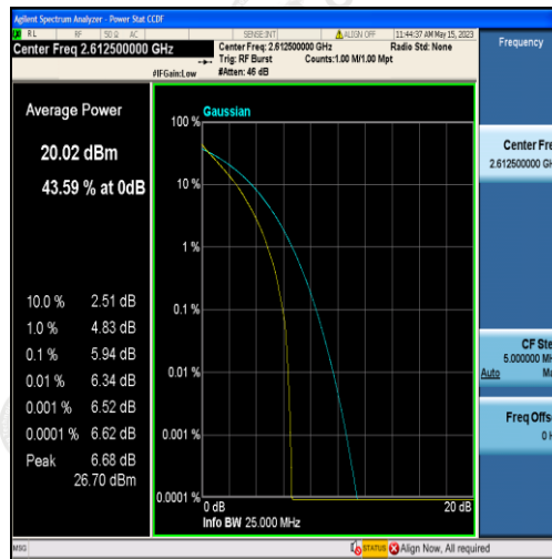
Band38-15MHz-QPSK-38175-75RB#0
