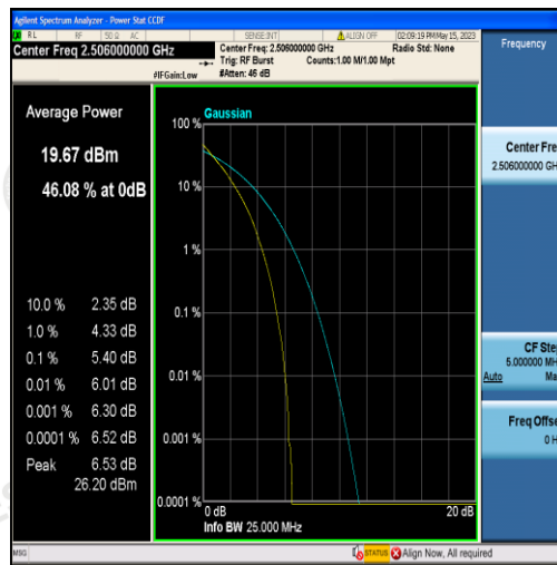
Band41-20MHz-QPSK-39750-100RB#0
