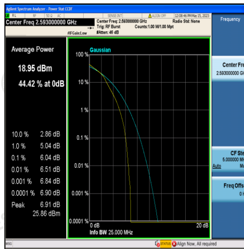
Band41-5MHz-16QAM-40620-25RB#0
