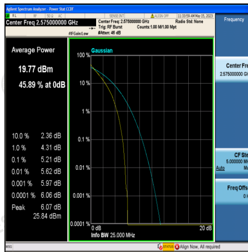
Band38-10MHz-QPSK-37800-50RB#0
