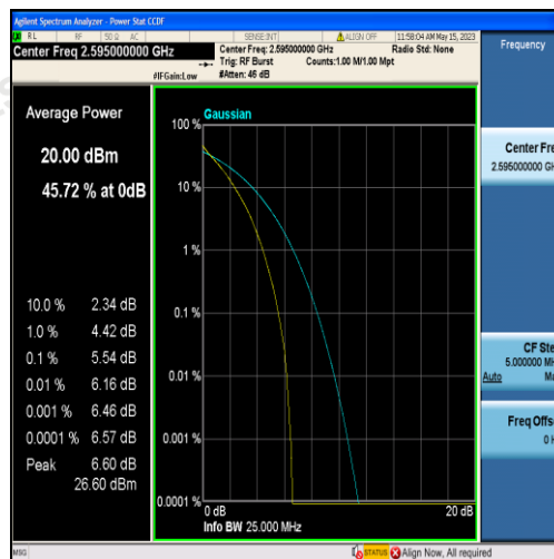
Band38-20MHz-QPSK-38000-100RB#0
