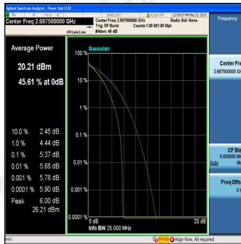
Band41-5MHz-QPSK-41565-25RB#0
