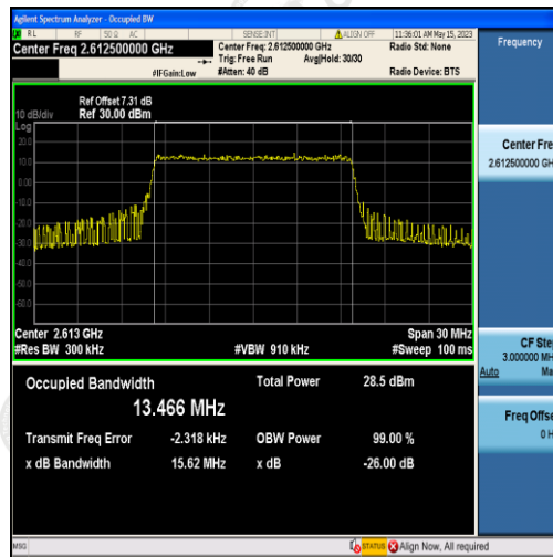
Band38-15MHz-QPSK-38175-75RB#0-13.466
