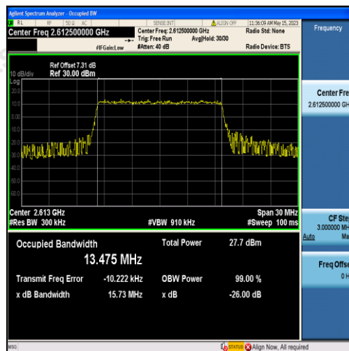
Band38-15MHz-16QAM-38175-75RB#0-13.475
