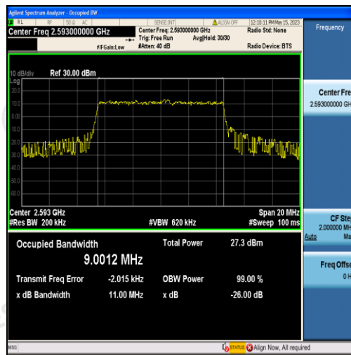
Band41-10MHz-16QAM-40620-50RB#0-9.0012
