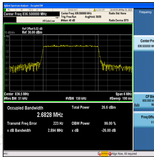
Band5-3MHz-16QAM-20525-15RB#0-2.6828
