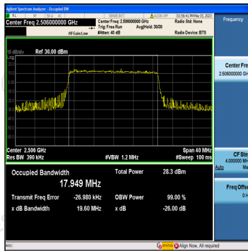
Band41-20MHz-QPSK-39750-100RB#0-17.949
