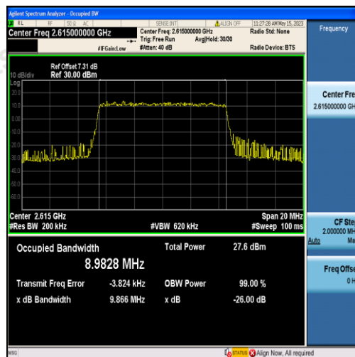
Band38-10MHz-16QAM-38200-50RB#0-8.9828
