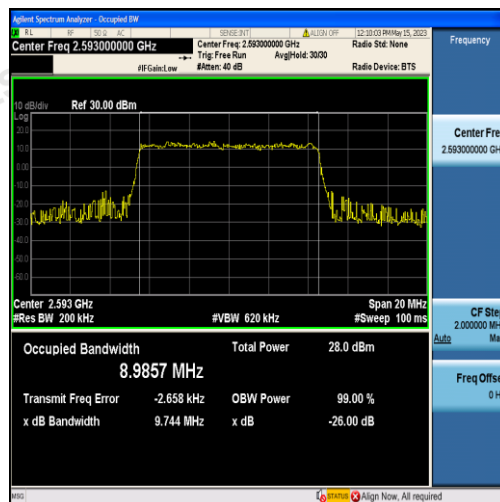
Band41-10MHz-QPSK-40620-50RB#0-8.9857
