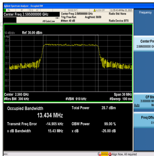
Band38-15MHz-QPSK-38000-75RB#0-13.434
