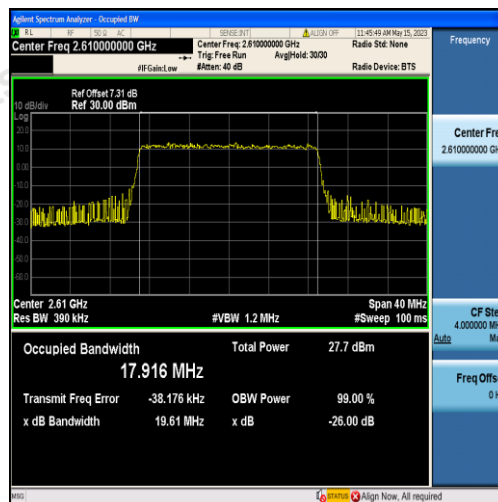
Band38-20MHz-16QAM-38150-100RB#0-17.916
