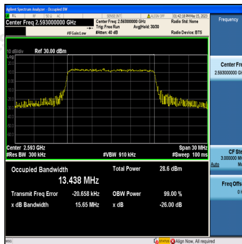
Band41-15MHz-QPSK-40620-75RB#0-13.438
