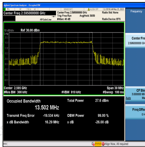
Band38-15MHz-16QAM-38000-75RB#0-13.502
