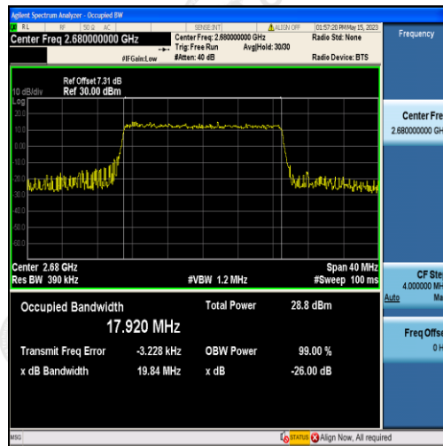
Band41-20MHz-QPSK-41490-100RB#0-17.920
