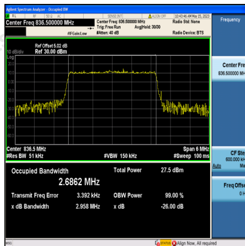
Band5-3MHz-QPSK-20525-15RB#0-2.6862
