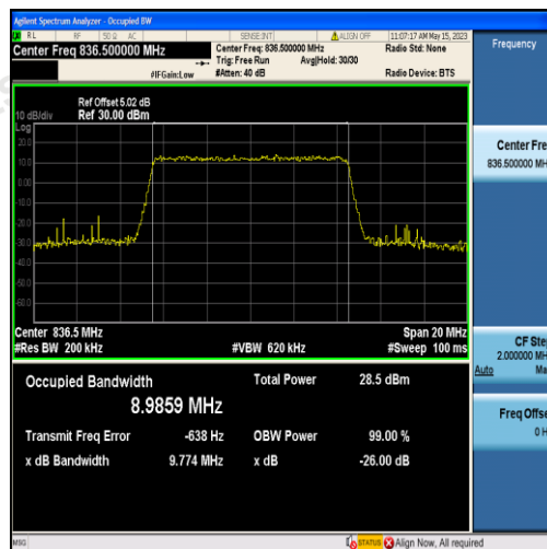
Band5-10MHz-QPSK-20525-50RB#0-8.9859
