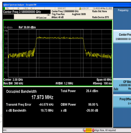
Band38-20MHz-QPSK-37850-100RB#0-17.973
