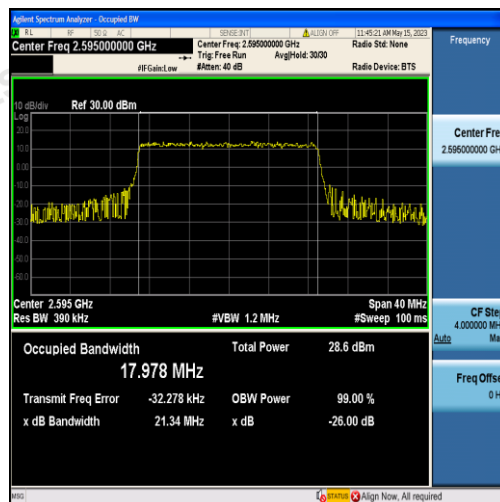
Band38-20MHz-QPSK-38000-100RB#0-17.978
