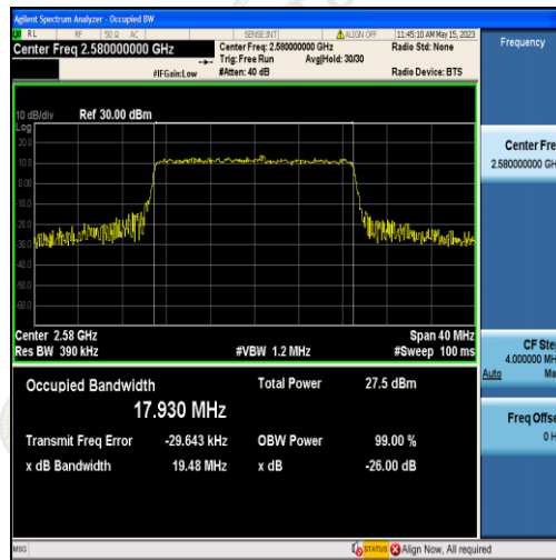
Band38-20MHz-16QAM-37850-100RB#0-17.930
