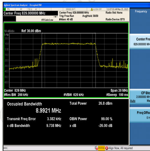
Band5-10MHz-16QAM-20450-50RB#0-8.9921
