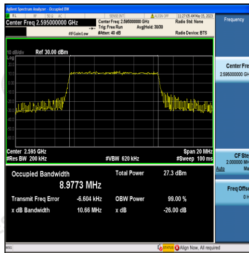
Band38-10MHz-16QAM-38000-50RB#0-8.9773
