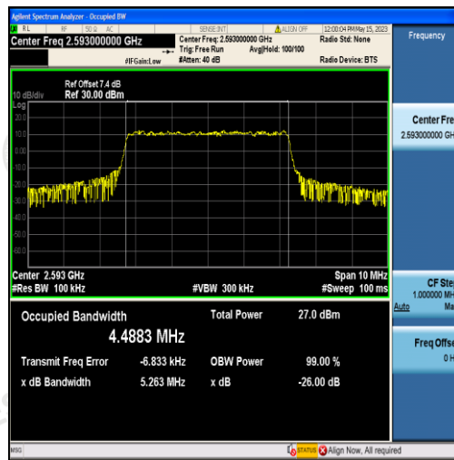
Band41-5MHz-16QAM-40620-25RB#0-4.4883
