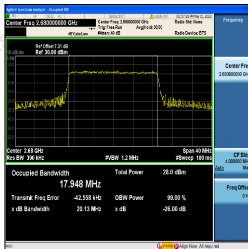
Band41-20MHz-16QAM-41490-100RB#0-17.948
