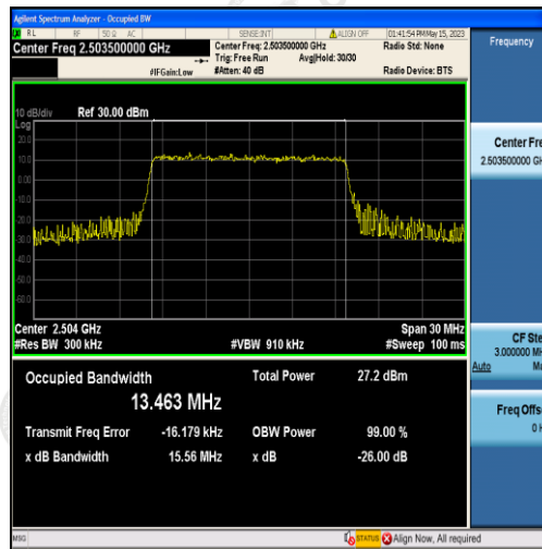
Band41-15MHz-16QAM-39725-75RB#0-13.463
