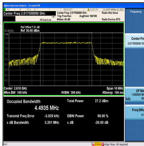
Band38-5MHz-16QAM-38225-25RB#0-4.4935
