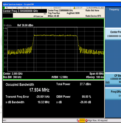
Band38-20MHz-16QAM-38000-100RB#0-17.934
