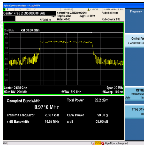
Band38-10MHz-QPSK-38000-50RB#0-8.9716
