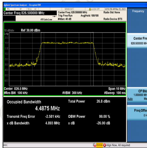
Band5-5MHz-16QAM-20425-25RB#0-4.4875
