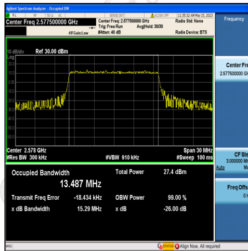
Band38-15MHz-16QAM-37825-75RB#0-13.487
