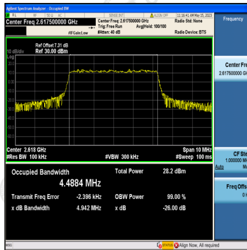
Band38-5MHz-QPSK-38225-25RB#0-4.4884
