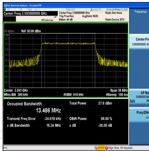
Band41-15MHz-16QAM-40620-75RB#0-13.486
