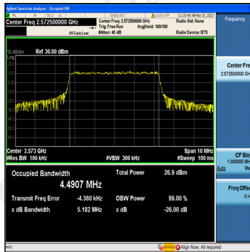
Band38-5MHz-16QAM-37775-25RB#0-4.4907
