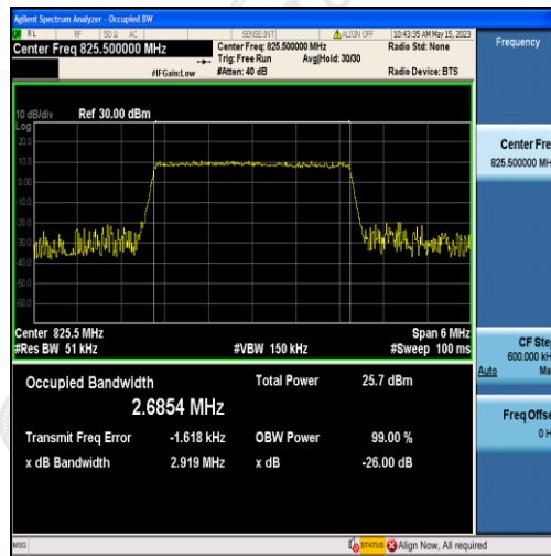
Band5-3MHz-16QAM-20415-15RB#0-2.6854
