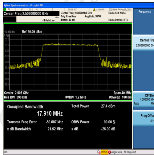
Band41-20MHz-16QAM-39750-100RB#0-17.910
