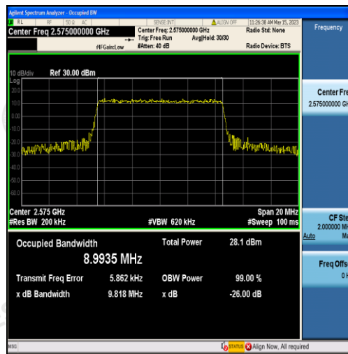
Band38-10MHz-QPSK-37800-50RB#0-8.9935
