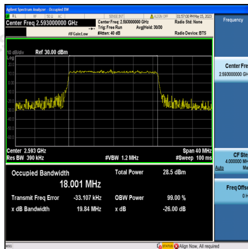
Band41-20MHz-QPSK-40620-100RB#0-18.001
