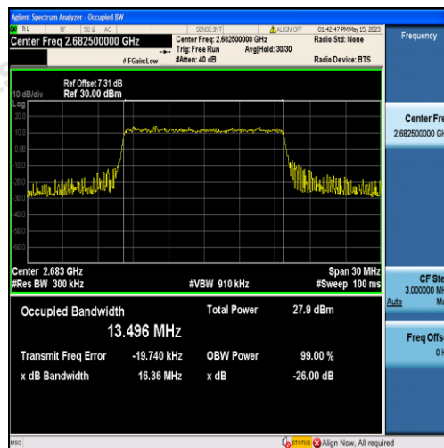
Band41-15MHz-16QAM-41515-75RB#0-13.496
