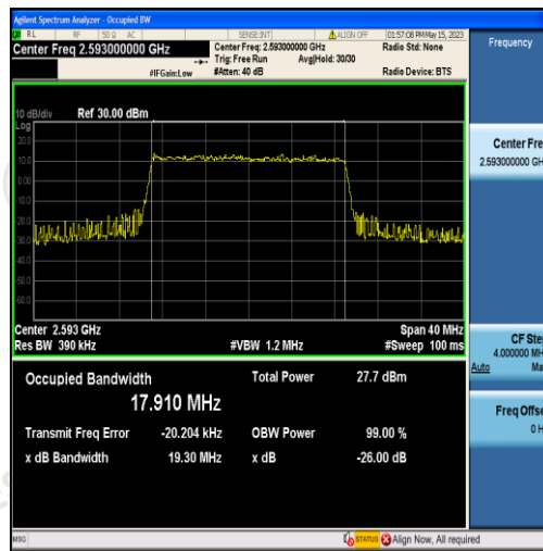
Band41-20MHz-16QAM-40620-100RB#0-17.910
