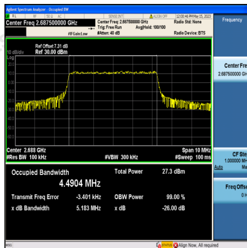
Band41-5MHz-16QAM-41565-25RB#0-4.4904
