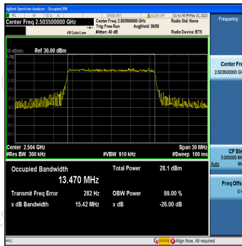
Band41-15MHz-QPSK-39725-75RB#0-13.470
