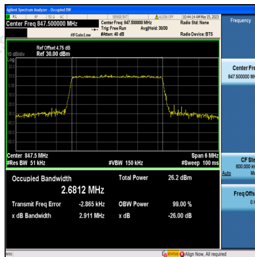
Band5-3MHz-16QAM-20635-15RB#0-2.6812
