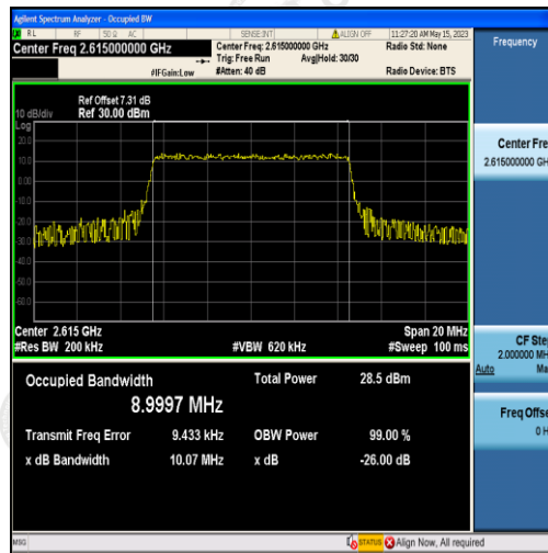
Band38-10MHz-QPSK-38200-50RB#0-8.9997
