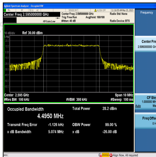
Band38-5MHz-QPSK-38000-25RB#0-4.4950
