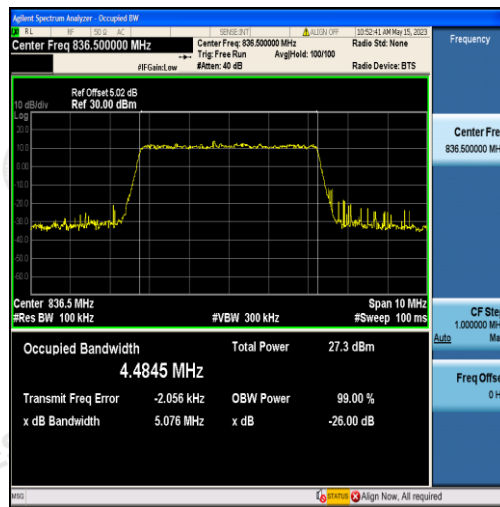
Band5-5MHz-16QAM-20525-25RB#0-4.4845
