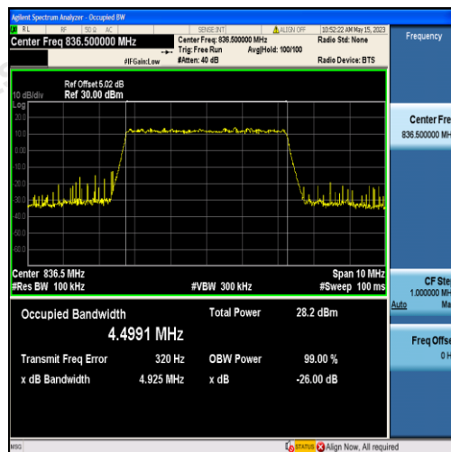
Band5-5MHz-QPSK-20525-25RB#0-4.4991
