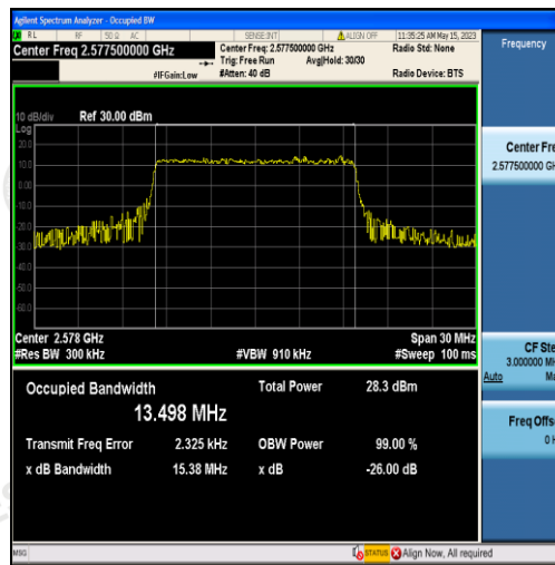
Band38-15MHz-QPSK-37825-75RB#0-13.498
