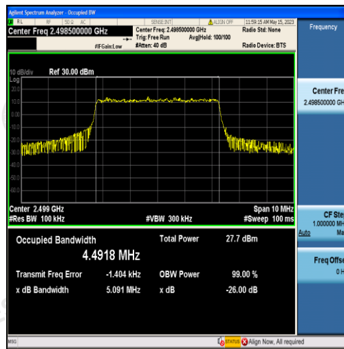
Band41-5MHz-QPSK-39675-25RB#0-4.4918
