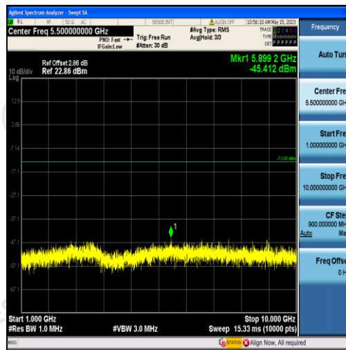
Band5-5MHz-QPSK-20425-25RB#0-Range2:1000~10000MHz
