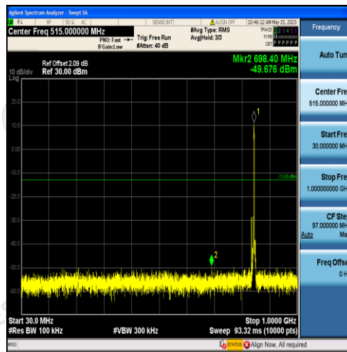
Band5-3MHz-16QAM-20635-15RB#0-Range1:30~1000MHz
