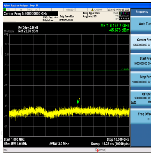
Band5-1.4MHz-16QAM-20525-6RB#0-Range2:1000~10000MHz
