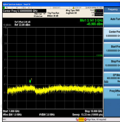
Band5-3MHz-16QAM-20525-15RB#0-Range2:1000~10000MHz
