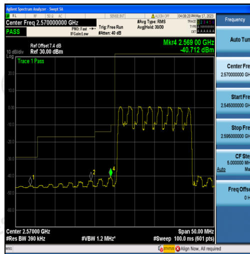
Band38-20MHz-16QAM-37850-100RB#0
