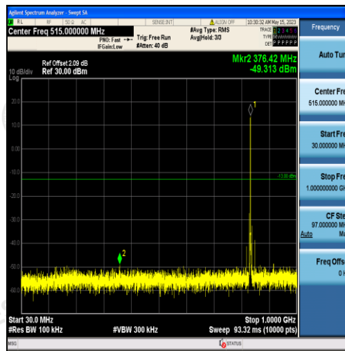
Band5-1.4MHz-QPSK-20525-6RB#0-Range1:30~1000MHz
