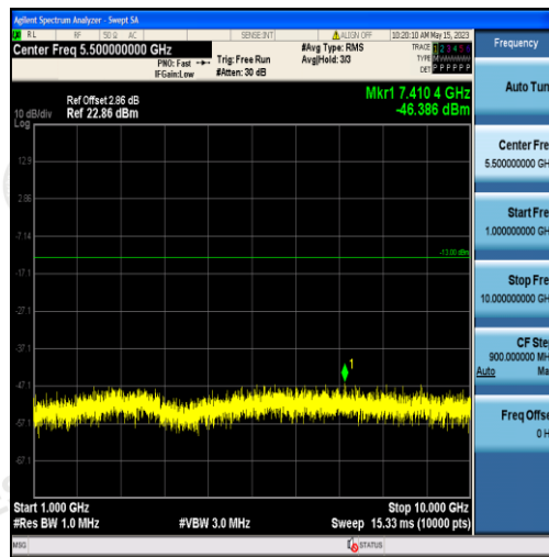
Band5-1.4MHz-QPSK-20407-6RB#0-Range2:1000~10000MHz
