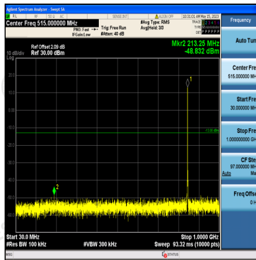
Band5-1.4MHz-16QAM-20643-6RB#0-Range1:30~1000MHz
