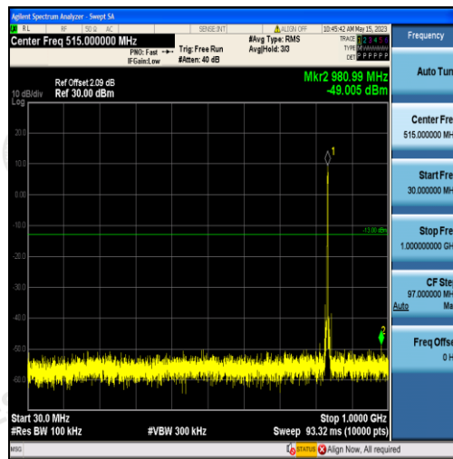
Band5-3MHz-QPSK-20525-15RB#0-Range1:30~1000MHz
