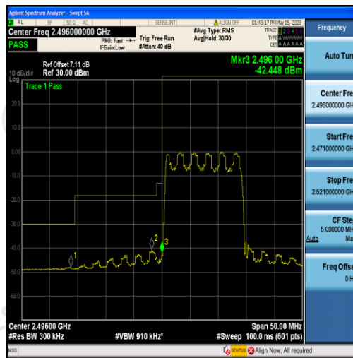
Band41-15MHz-16QAM-39725-75RB#0
