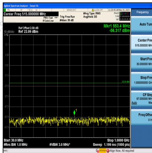
Band38-10MHz-16QAM-38000-50RB#0-Range1:30~1000MHz
