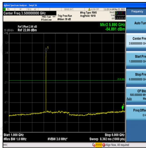
Band38-5MHz-16QAM-38000-25RB#0-Range2:1000~6000MHz
