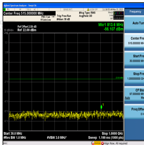
Band38-15MHz-16QAM-38000-75RB#0-Range1:30~1000MHz
