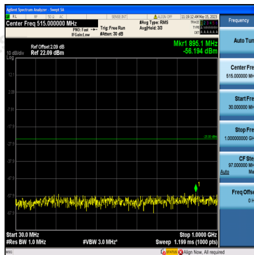
Band38-5MHz-16QAM-37775-25RB#0-Range1:30~1000MHz
