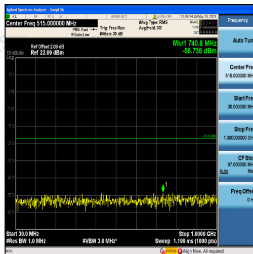
Band38-15MHz-QPSK-38000-75RB#0-Range1:30~1000MHz
