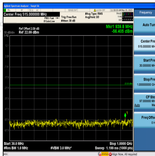
Band38-10MHz-QPSK-38200-50RB#0-Range1:30~1000MHz
