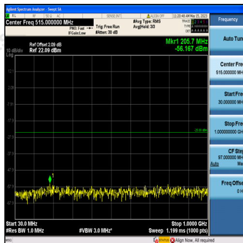
Band38-5MHz-16QAM-38225-25RB#0-Range1:30~1000MHz
