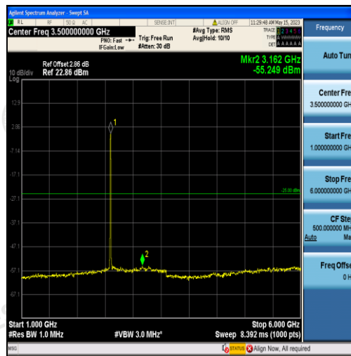
Band38-10MHz-16QAM-38000-50RB#0-Range2:1000~6000MHz
