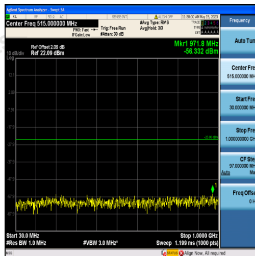
Band38-15MHz-16QAM-37825-75RB#0-Range1:30~1000MHz
