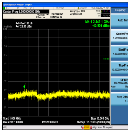
Band5-10MHz-QPSK-20450-50RB#0-Range2:1000~10000MHz
