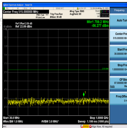
Band38-15MHz-QPSK-38175-75RB#0-Range1:30~1000MHz
