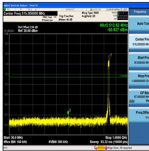
Band5-10MHz-16QAM-20600-50RB#0-Range1:30~1000MHz
