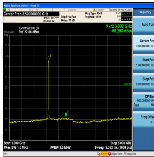
Band38-15MHz-16QAM-38000-75RB#0-Range2:1000~6000MHz
