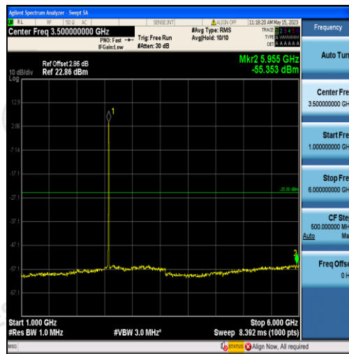
Band38-5MHz-QPSK-37775-25RB#0-Range2:1000~6000MHz
