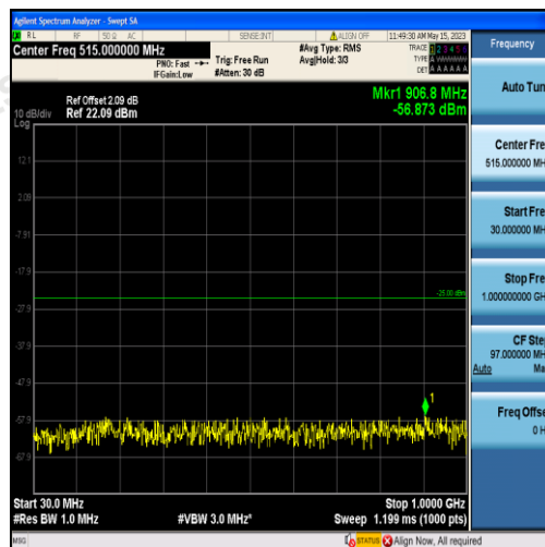
Band38-20MHz-QPSK-38000-100RB#0-Range1:30~1000MHz
