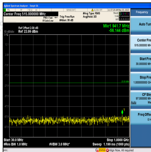
Band38-15MHz-QPSK-37825-75RB#0-Range1:30~1000MHz
