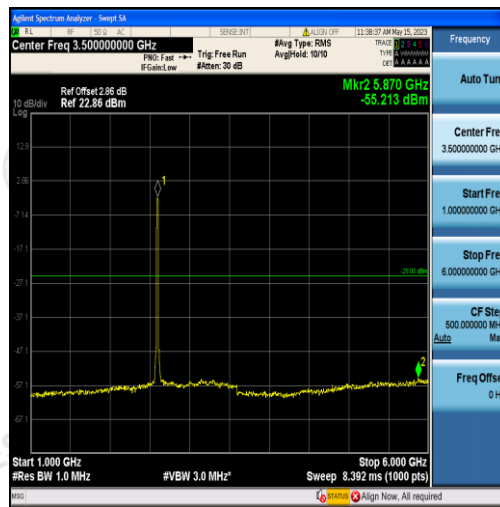
Band38-15MHz-QPSK-38000-75RB#0-Range2:1000~6000MHz
