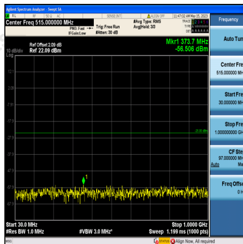
Band38-20MHz-QPSK-37850-100RB#0-Range1:30~1000MHz
