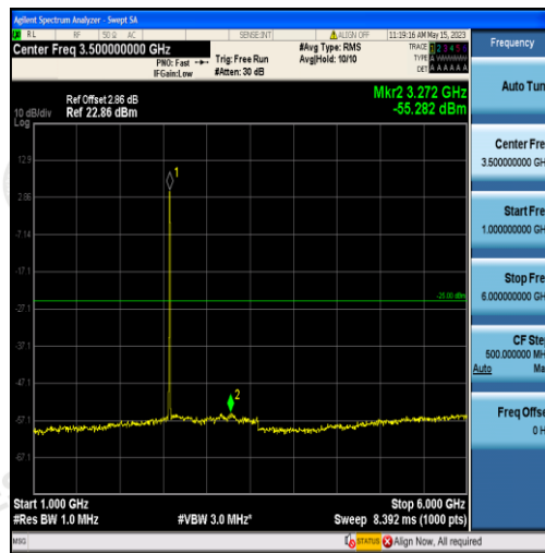
Band38-5MHz-16QAM-37775-25RB#0-Range2:1000~6000MHz
