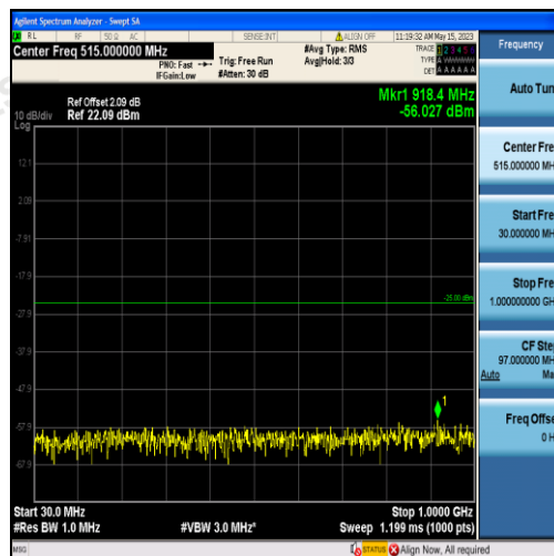
Band38-5MHz-QPSK-38000-25RB#0-Range1:30~1000MHz
