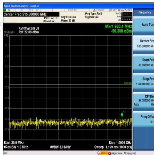
Band38-5MHz-QPSK-37775-25RB#0-Range1:30~1000MHz
