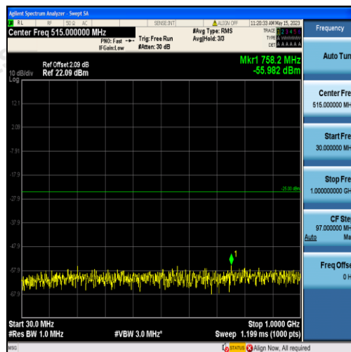
Band38-5MHz-QPSK-38225-25RB#0-Range1:30~1000MHz
