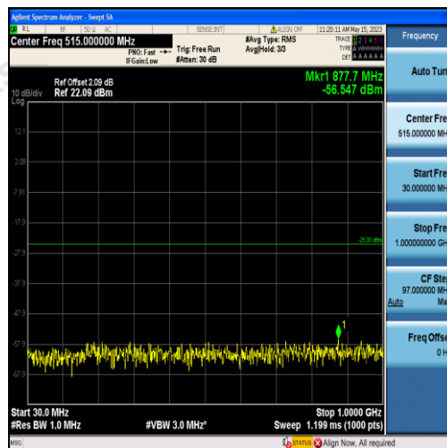
Band38-5MHz-16QAM-38000-25RB#0-Range1:30~1000MHz
