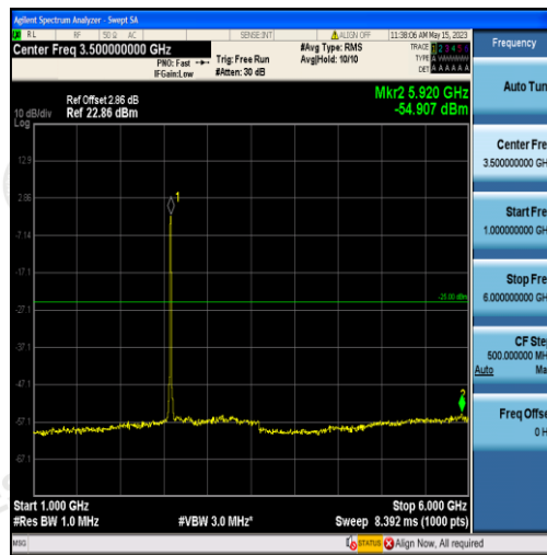
Band38-15MHz-16QAM-37825-75RB#0-Range2:1000~6000MHz
