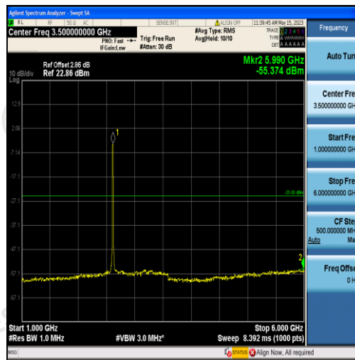
Band38-15MHz-16QAM-38175-75RB#0-Range2:1000~6000MHz
