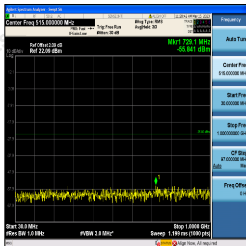
Band38-10MHz-QPSK-37800-50RB#0-Range1:30~1000MHz
