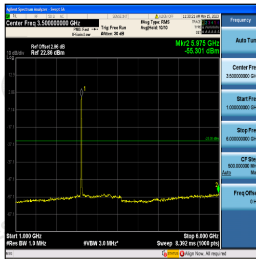
Band38-10MHz-16QAM-38200-50RB#0-Range2:1000~6000MHz
