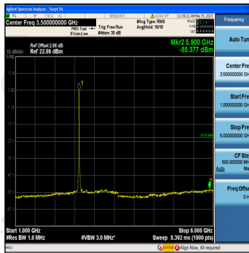
Band38-15MHz-QPSK-38175-75RB#0-Range2:1000~6000MHz
