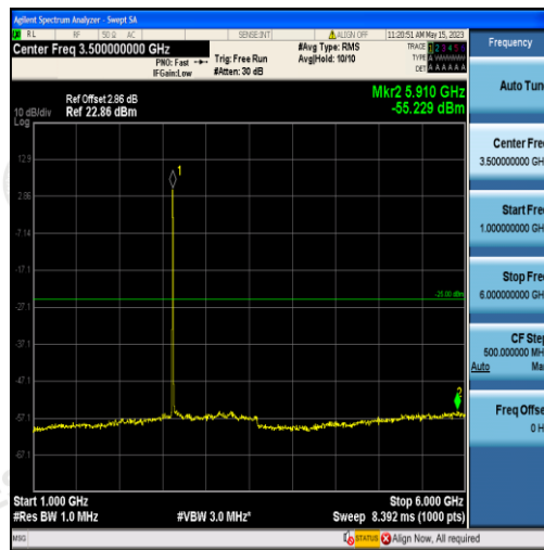
Band38-5MHz-16QAM-38225-25RB#0-Range2:1000~6000MHz
