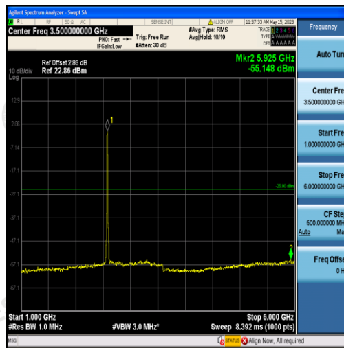
Band38-15MHz-QPSK-37825-75RB#0-Range2:1000~6000MHz
