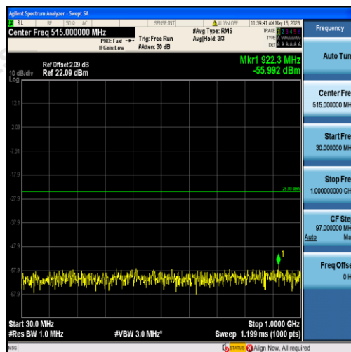
Band38-15MHz-16QAM-38175-75RB#0-Range1:30~1000MHz
