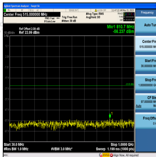
Band38-20MHz-16QAM-37850-100RB#0-Range1:30~1000MHz
