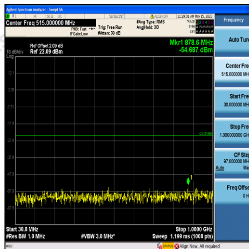
Band38-10MHz-16QAM-37800-50RB#0-Range1:30~1000MHz
