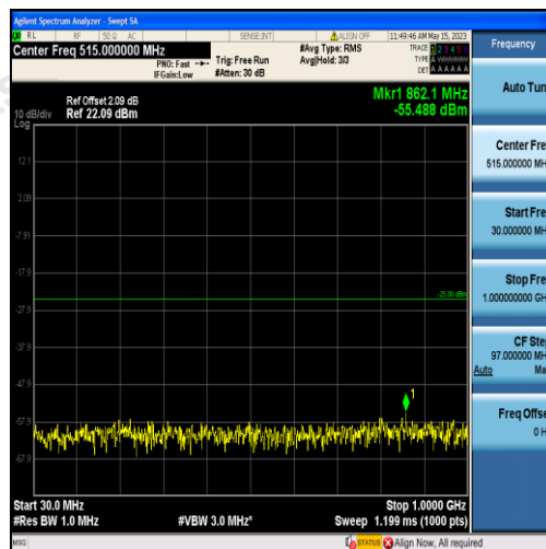
Band38-20MHz-16QAM-38000-100RB#0-Range1:30~1000MHz
