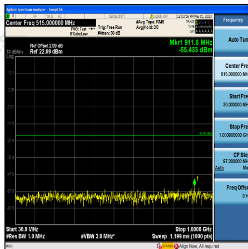
Band41-5MHz-16QAM-40620-25RB#0-Range1:30~1000MHz
