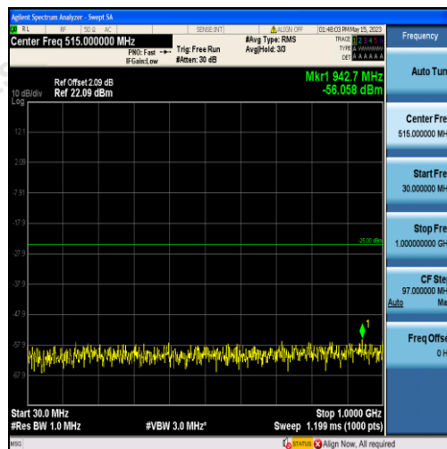
Band41-15MHz-16QAM-39725-75RB#0-Range1:30~1000MHz
