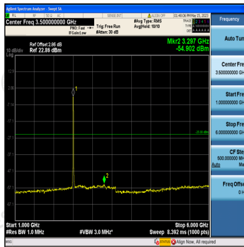
Band41-15MHz-16QAM-39725-75RB#0-Range2:1000~6000MHz
