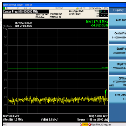
Band41-5MHz-16QAM-41565-25RB#0-Range1:30~1000MHz
