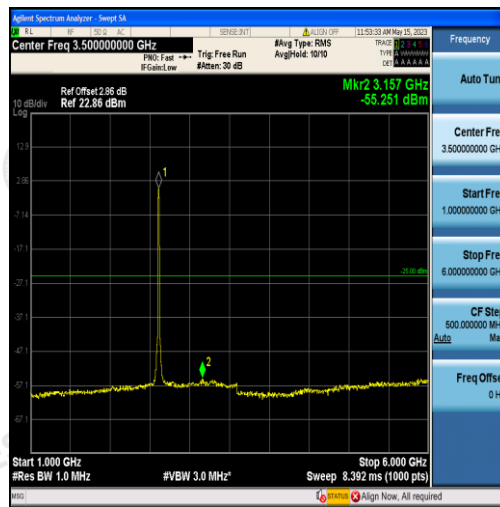
Band38-20MHz-16QAM-38150-100RB#0-Range2:1000~6000MHz
