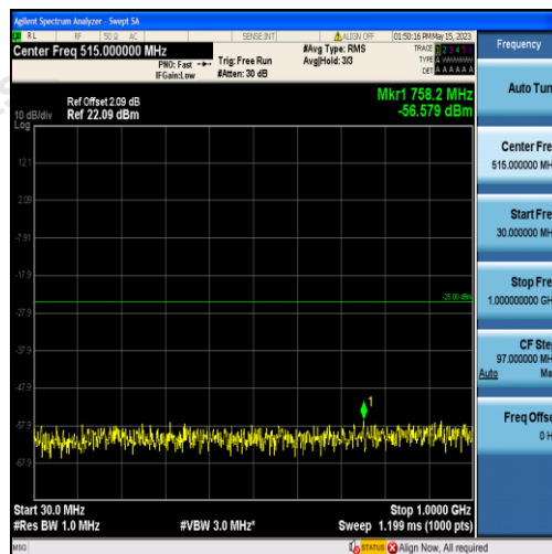
Band41-15MHz-QPSK-41515-75RB#0-Range1:30~1000MHz
