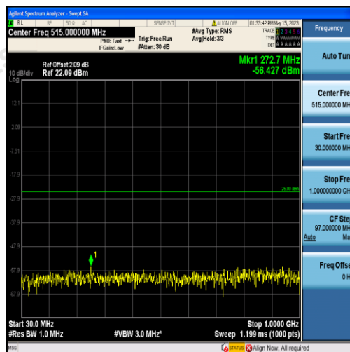
Band41-10MHz-16QAM-39700-50RB#0-Range1:30~1000MHz
