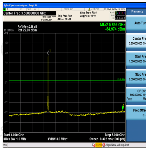
Band41-15MHz-16QAM-41515-75RB#0-Range2:1000~6000MHz
