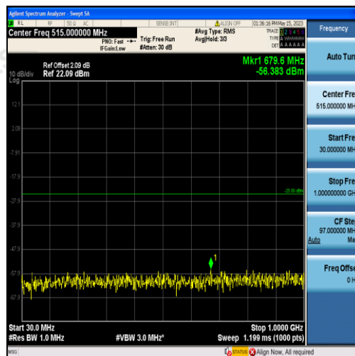
Band41-10MHz-16QAM-41540-50RB#0-Range1:30~1000MHz
