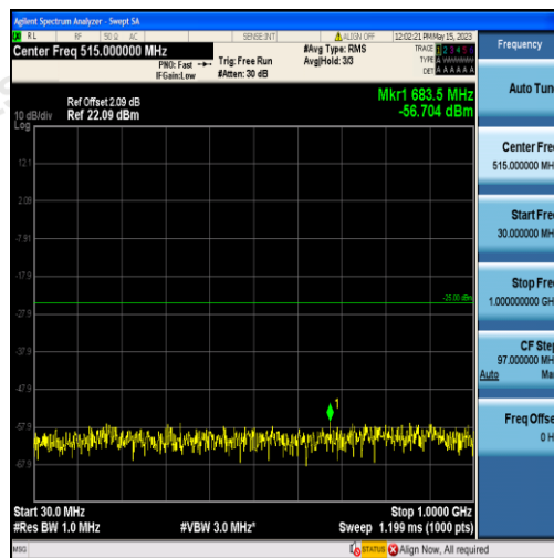
Band41-5MHz-16QAM-39675-25RB#0-Range1:30~1000MHz
