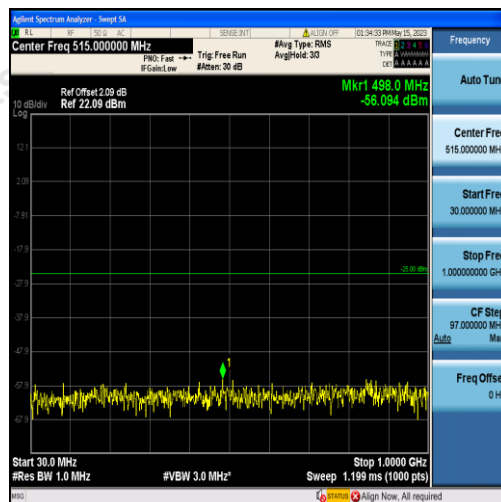
Band41-10MHz-16QAM-40620-50RB#0-Range1:30~1000MHz
