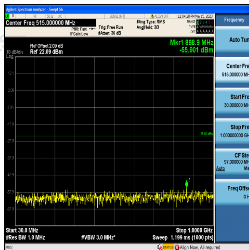
Band41-5MHz-QPSK-41565-25RB#0-Range1:30~1000MHz
