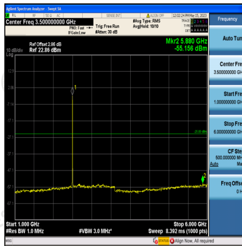
Band41-5MHz-16QAM-39675-25RB#0-Range2:1000~6000MHz
