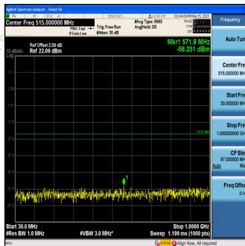
Band41-15MHz-QPSK-39725-75RB#0-Range1:30~1000MHz
