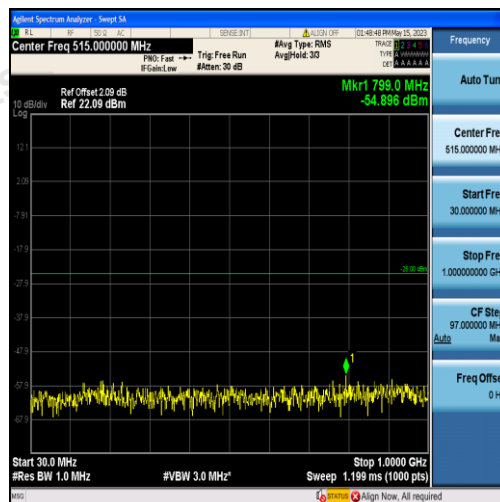
Band41-15MHz-QPSK-40620-75RB#0-Range1:30~1000MHz
