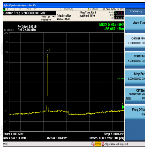
Band41-20MHz-16QAM-41490-100RB#0-Range2:1000~6000MHz
