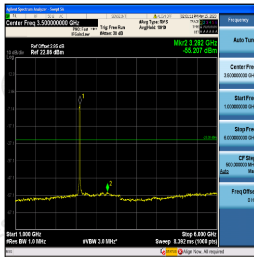
Band41-20MHz-16QAM-40620-100RB#0-Range2:1000~6000MHz
