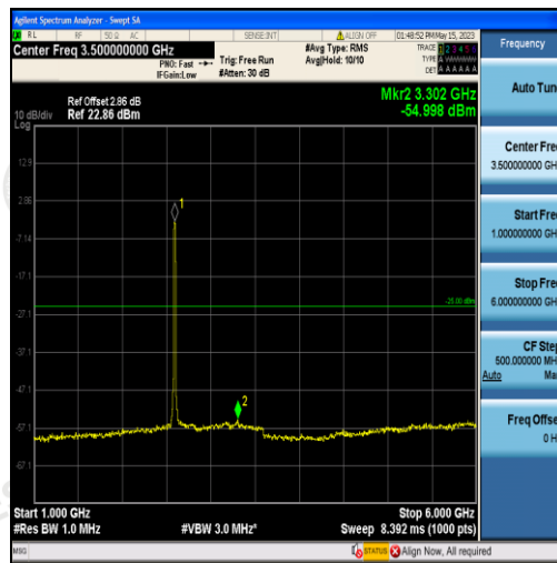
Band41-15MHz-QPSK-40620-75RB#0-Range2:1000~6000MHz
