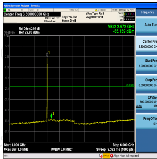
Band41-15MHz-QPSK-39725-75RB#0-Range2:1000~6000MHz
