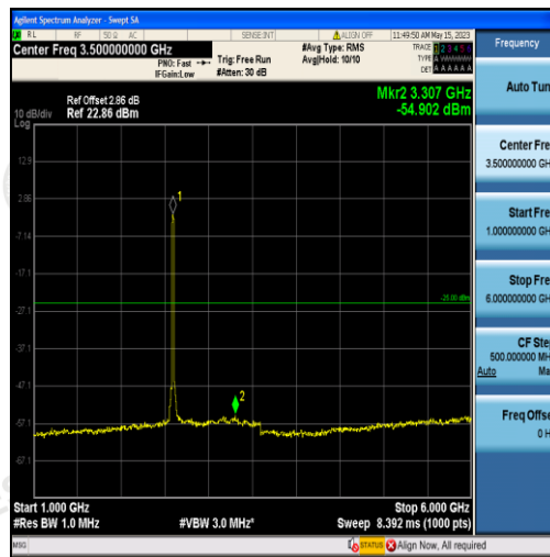
Band38-20MHz-16QAM-38000-100RB#0-Range2:1000~6000MHz
