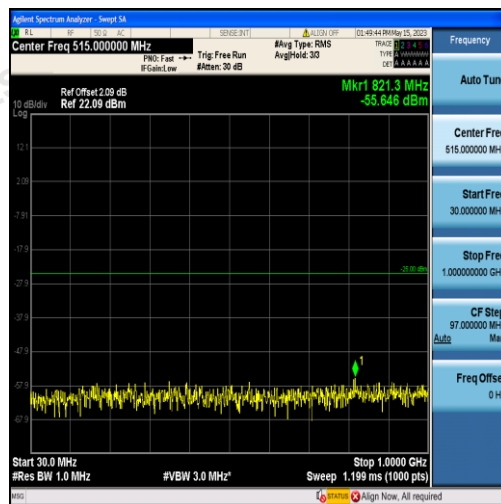
Band41-15MHz-16QAM-40620-75RB#0-Range1:30~1000MHz
