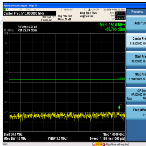
Band41-20MHz-QPSK-39750-100RB#0-Range1:30~1000MHz
