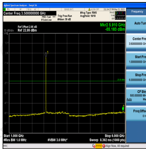
Band41-10MHz-16QAM-40620-50RB#0-Range2:1000~6000MHz
