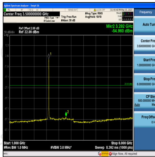
Band41-15MHz-16QAM-40620-75RB#0-Range2:1000~6000MHz
