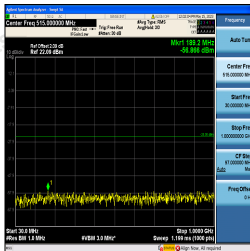
Band41-5MHz-QPSK-39675-25RB#0-Range1:30~1000MHz
