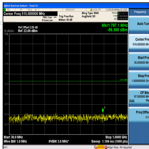
Band38-20MHz-16QAM-38150-100RB#0-Range1:30~1000MHz
