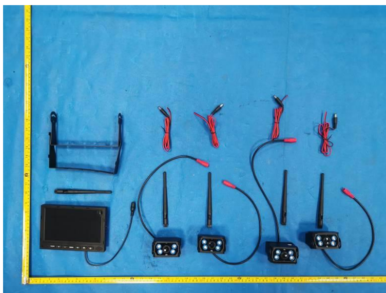
YB-N-Wireless-4 Photo 6
