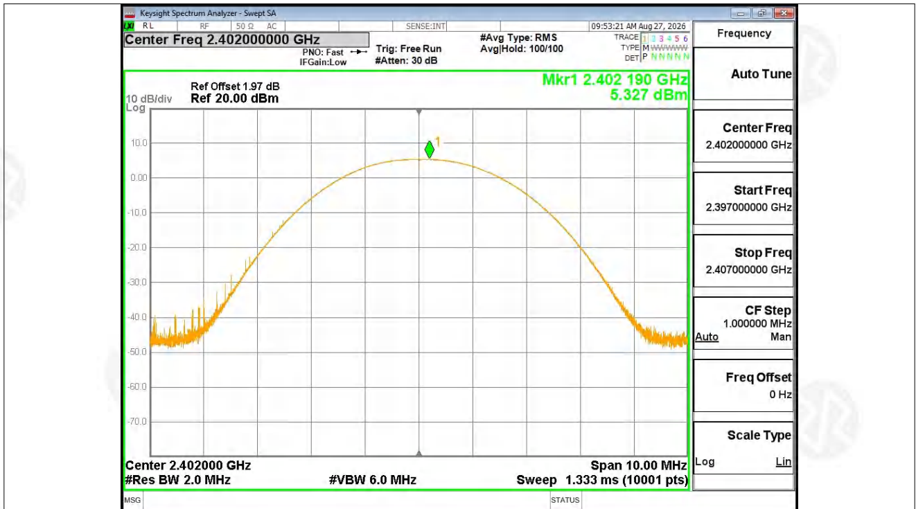
Peak Power NVNT 1-DH5 2402MHz Ant1
