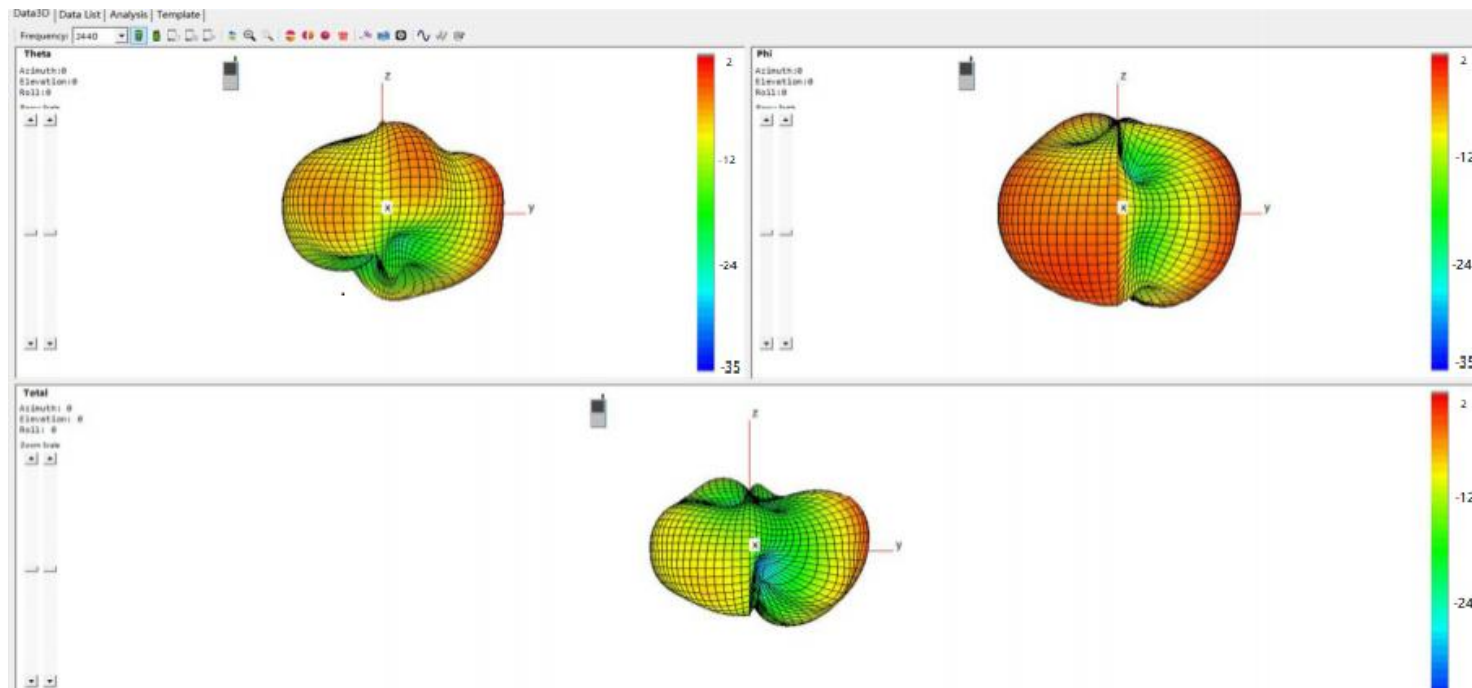
3D Radiation Pattern for 2440MHz
