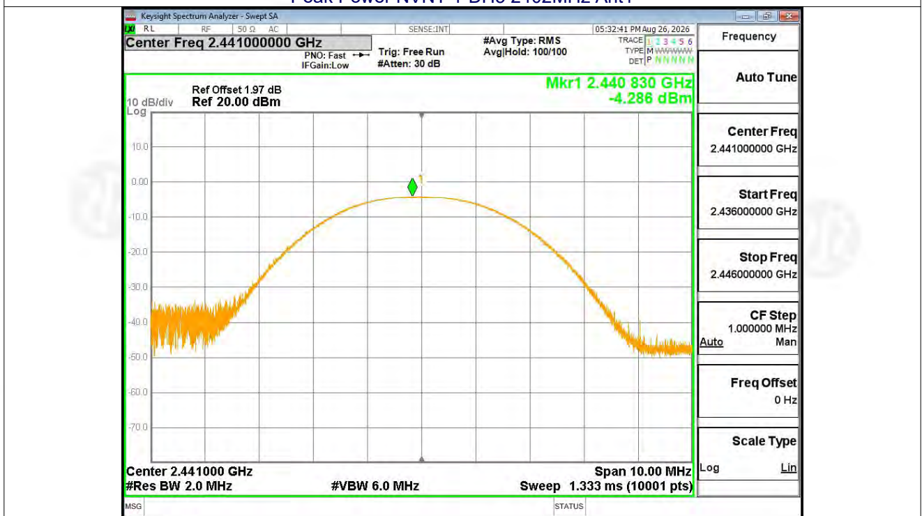
Peak Power NVNT 1-DH5 2441MHz Ant1
