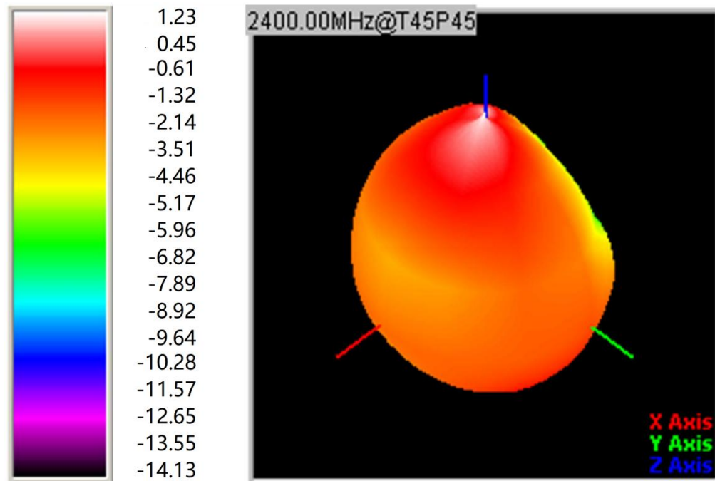
3D Radiation Pattern for 2400MHz
