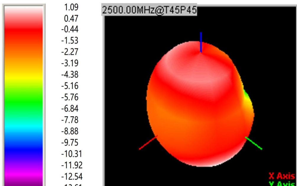
3D Radiation Pattern for 2500MHz
