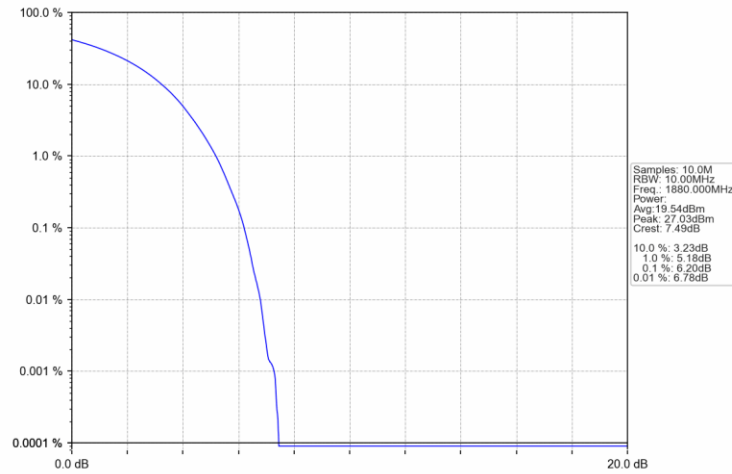
Band2 15MHz 16QAM MCH 1880MHz RB 27 0 NTNV
