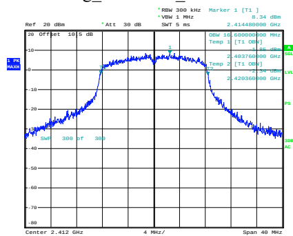
g_2412MHz_Chain 0
