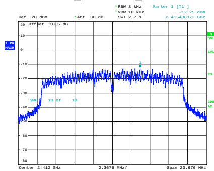
n20_2412MHz_Chain 0
