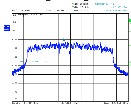
n20_2437MHz_Chain 0
