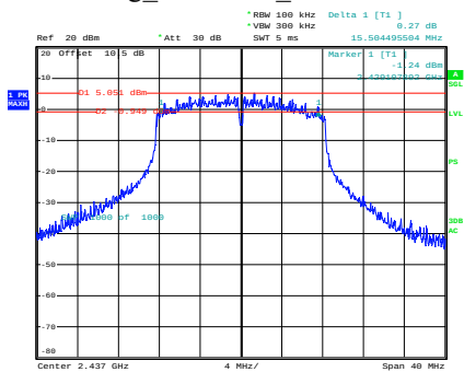
g_2437MHz_Chain 0
