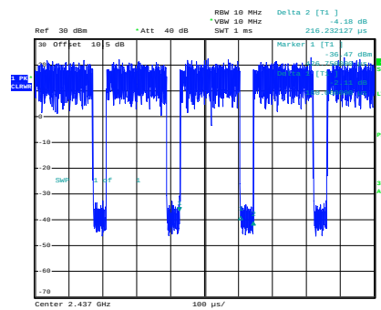
g_2437MHz_Chain 0
