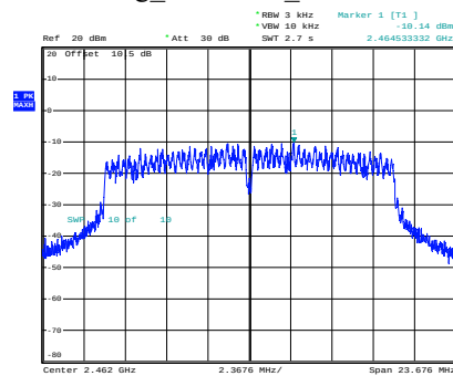
g_2462MHz_Chain 0
