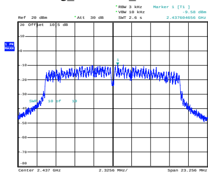
g_2437MHz_Chain 0
