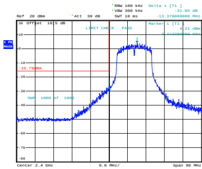
g_2412MHz_Chain 0
