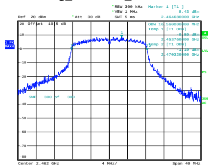
g_2462MHz_Chain 0
