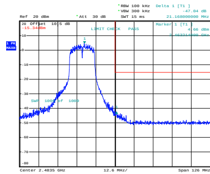
g_2462MHz_Chain 0
