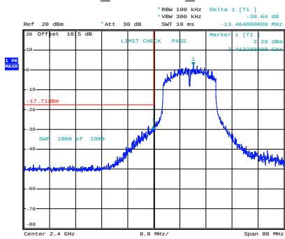
n20_2412MHz_Chain 0
