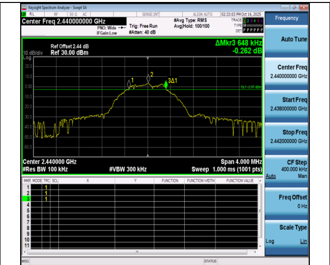
BLE_1M-Ant1-2440-PASS
