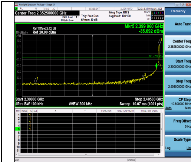
BLE_1M-Ant1-2402-PASS
