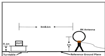
Below 30MHz
