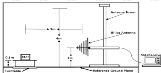
Below 1GHz
