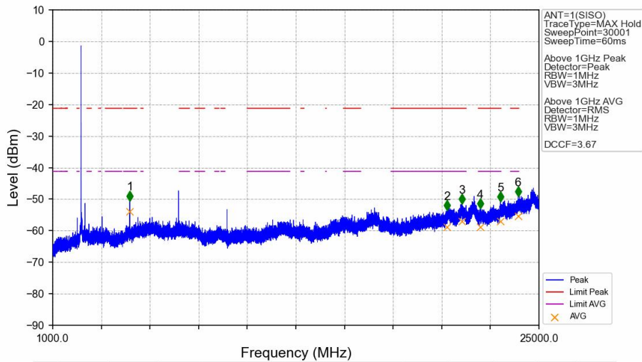
1M_LCH_2402MHz_Ant1_NTNV
