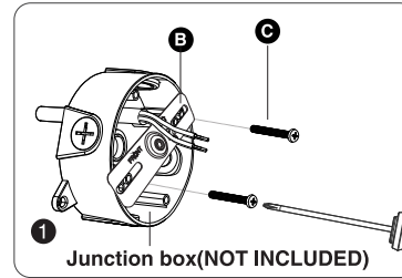
Junction box(NOT INCLUDED)
