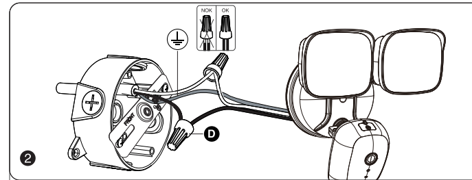
Junction box(NOT INCLUDED)
