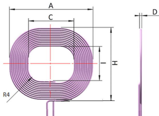
Coil 2
