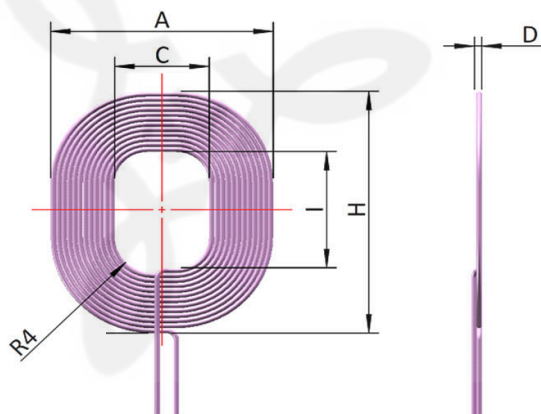
Coil 1&3
