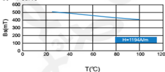
Bs—T Curve
