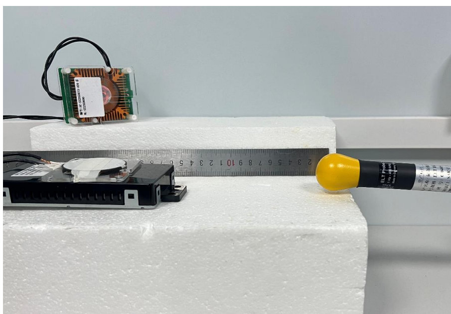
E-Field Test Setup Photo of Position B (15cm)
