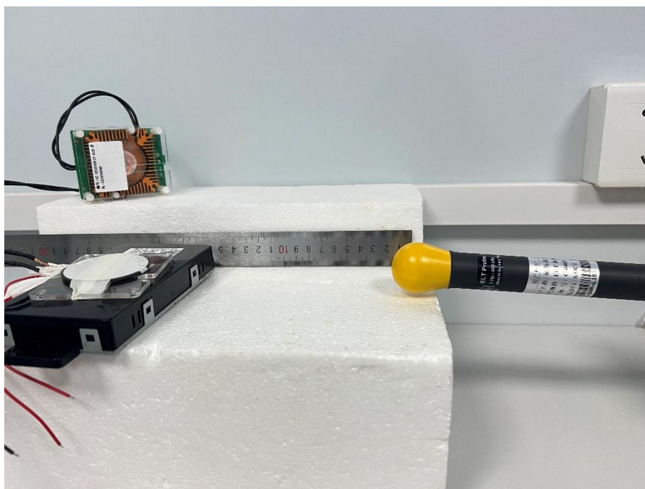
E-Field Test Setup Photo of Position D (15cm)
