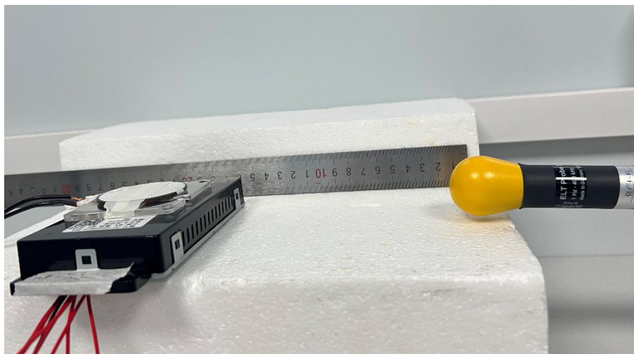
E-Field Test Setup Photo of Position C (15cm)
