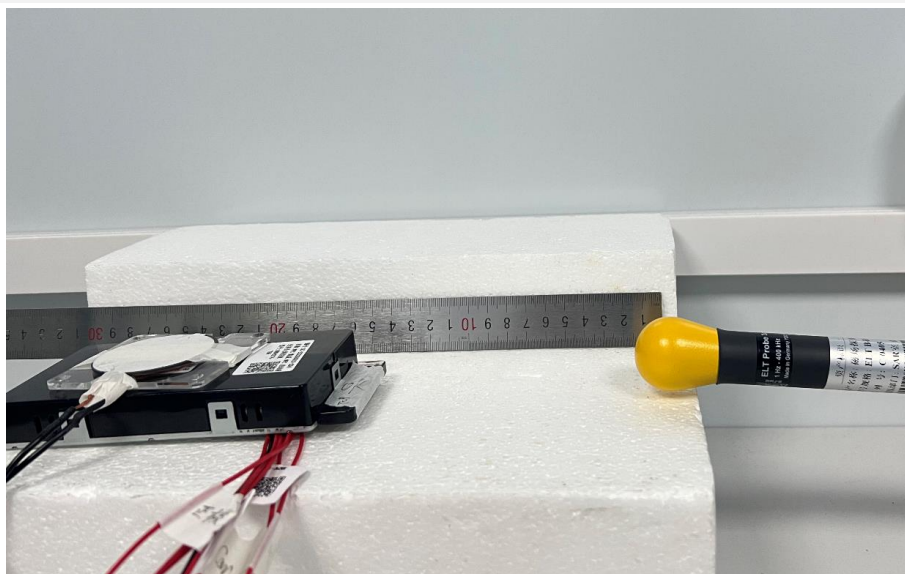
E-Field Test Setup Photo of Position A (15cm)
