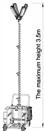
Working status of lighting fixtures
