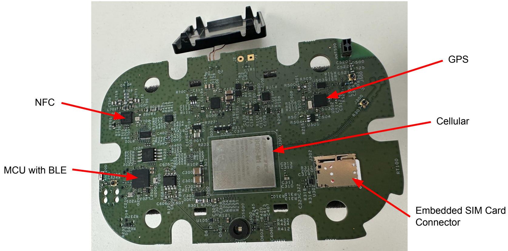
Main PCBA Front Side
