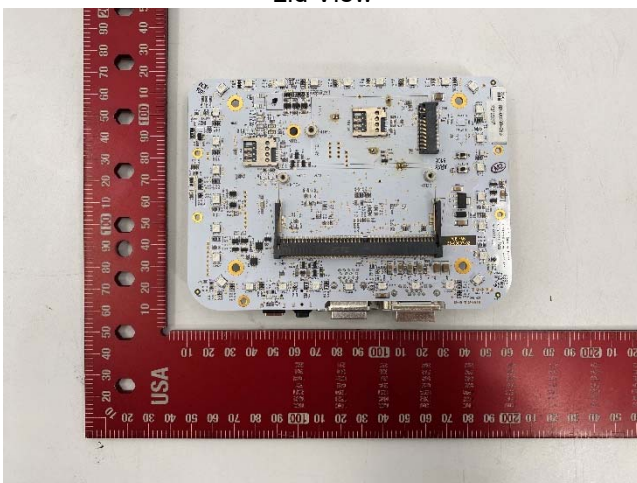
Main Board View 2
