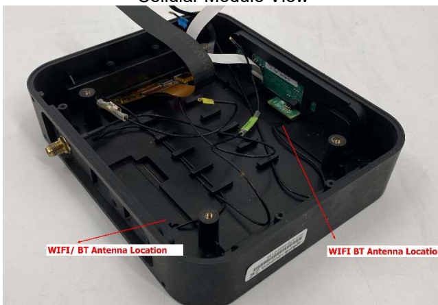
WLAN/ BT Antenna Location View
