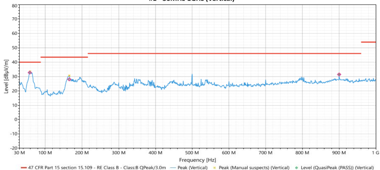
#1 - 30MHz-1GHz (Vertical)
